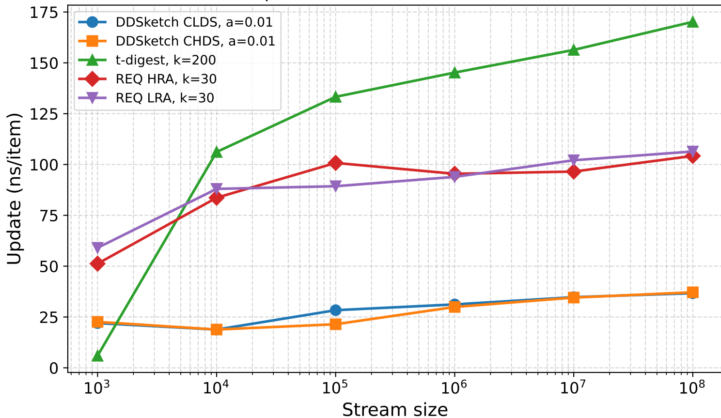
Update (ns/item), Pareto(1.5, 1)
