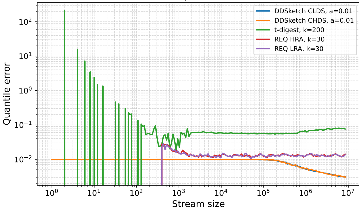
Quantile error, Exponential(1.5), level 0.5
