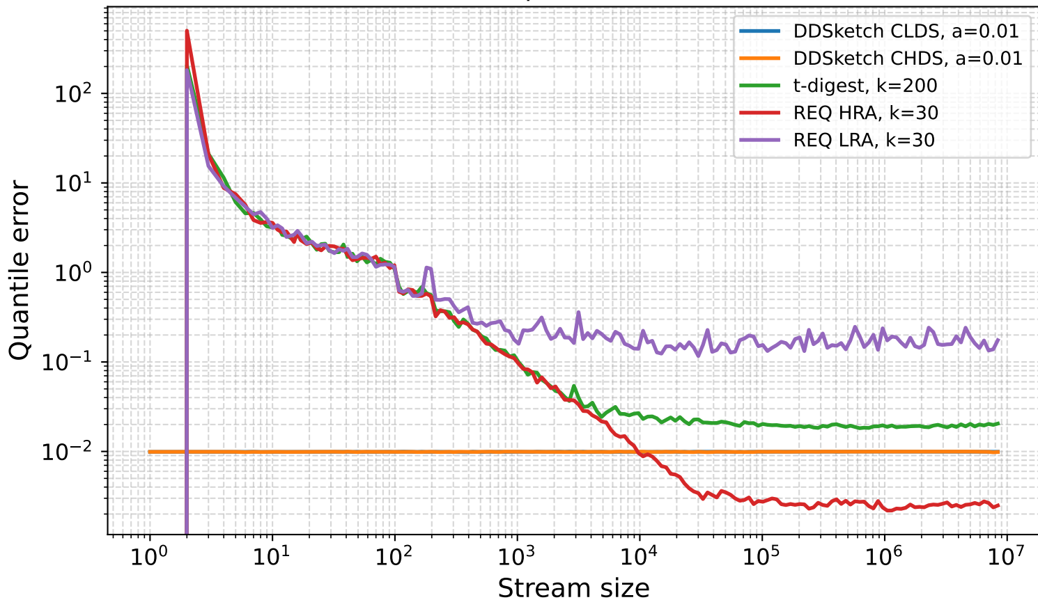
Quantile error, Exponential(1.5), level 0.99
