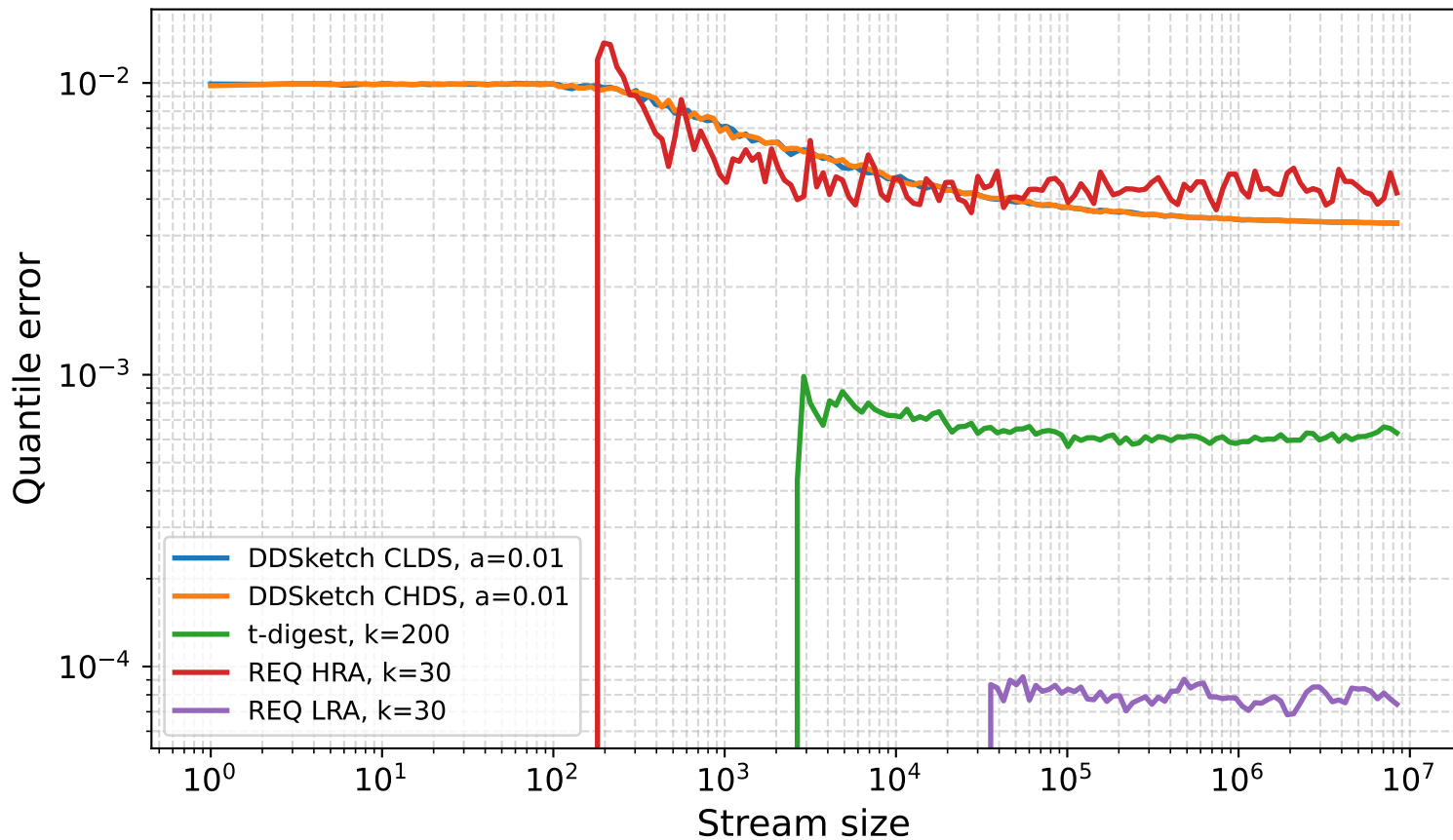
Quantile error, Pareto(1.5, 1), level 0.01
