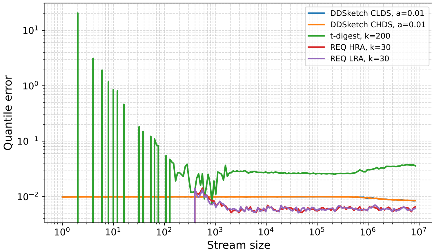
Quantile error, Pareto(1.5, 1), level 0.5
