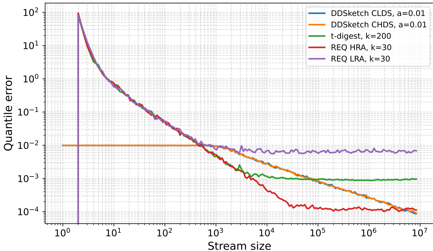
Quantile error, Uniform(0,1), level 0.99
