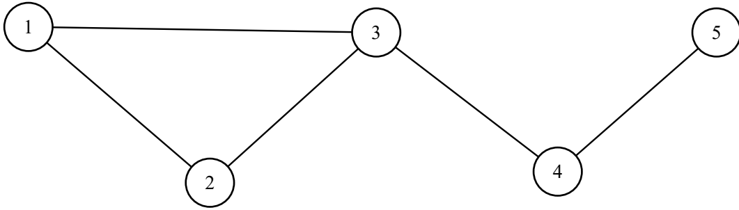
Figure 5. Graph G
