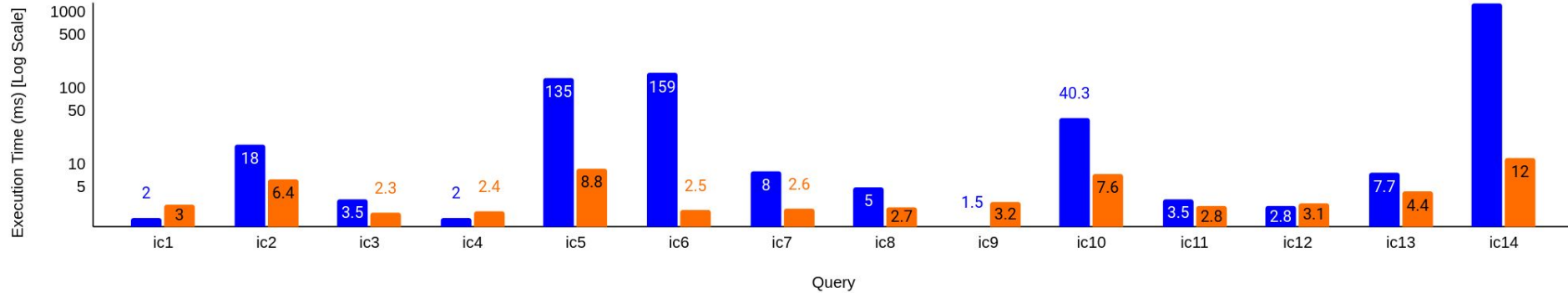
Neo4j vs TigerGraph for IC Queries with Scale Factor 0.1
