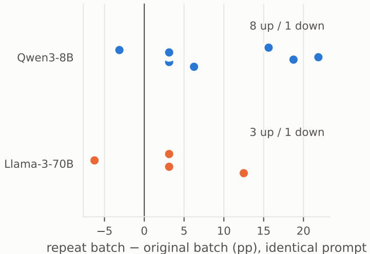
(b) The null control is not centred on zero for Qwen
