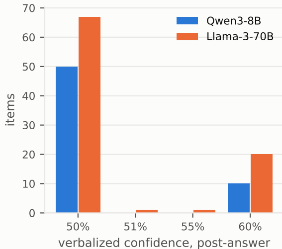
(a) Matching leaves confidence nearly binary
