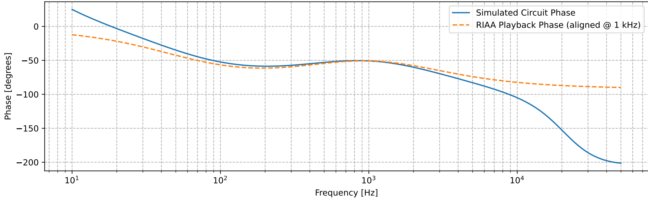
Phase Response Comparison (1 kHz aligned)
