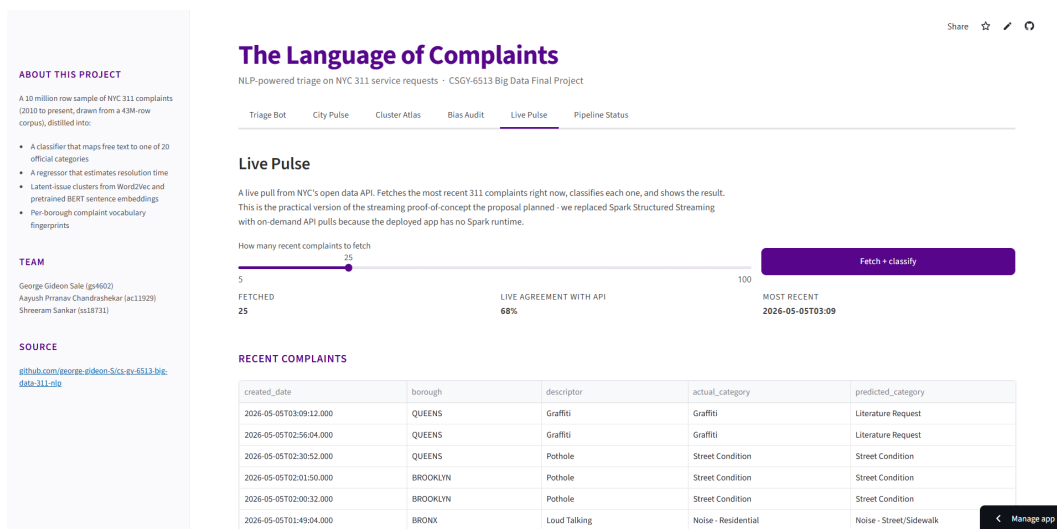
Figure 16: Live Pulse tab. The "Fetch + classify" button pulls the most recent N complaints from NYC's Open Data API on demand, classifies each one with the deployed model, and shows the result alongside the actual category for live agreement measurement. This is the practical replacement for the Spark Structured Streaming PoC the proposal originally planned: same end-state (live classification of incoming tickets), no Spark JVM at request time.
