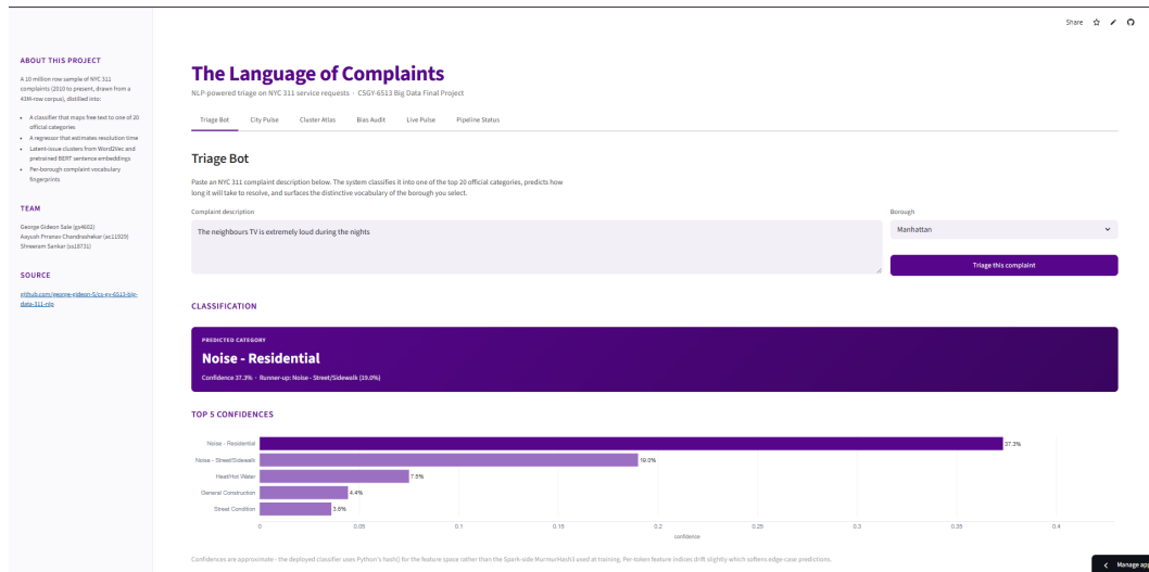
Figure 6: Triage Bot tab, upper half. The user pastes a complaint ("The neighbours TV is extremely loud during the nights"), picks a borough (Manhattan in this snapshot), and the served NumPy inference path returns a predicted category card and a top-5 confidences bar chart. Predicted category is Noise - Residential at 37.3 percent confidence with Noise - Street/Sidewalk as runner-up at 19.0 percent, which is the documented confusable pair from section 5.1.
