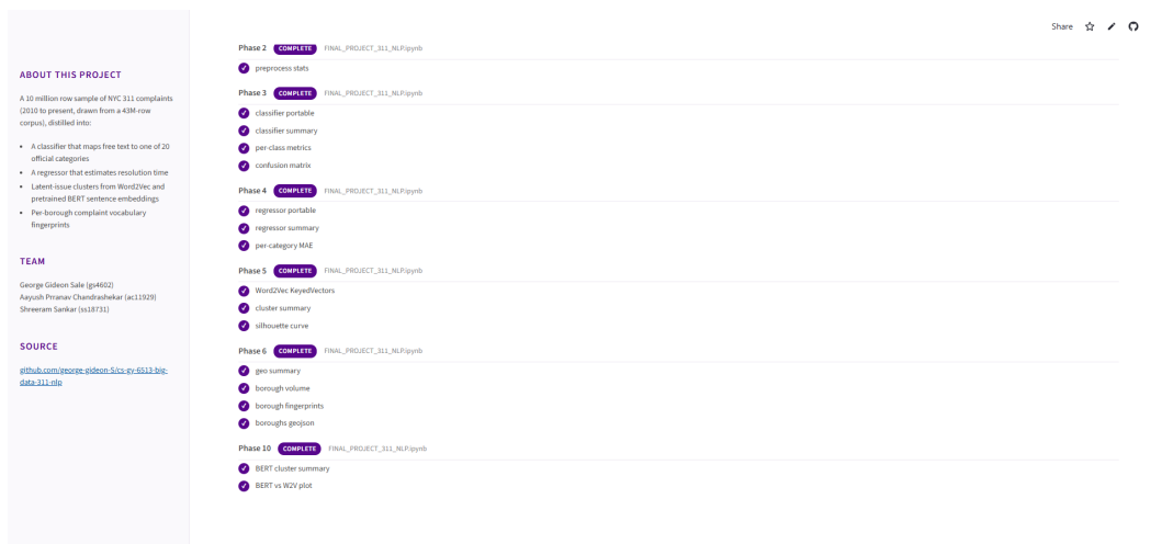
Figure 18: Pipeline Status tab, lower half. Continuation of the artifacts-by-phase block: every artifact from Phase 2 (preprocess stats) through Phase 10 (BERT cluster summary, BERT vs W2V plot) is marked complete in this snapshot. This is the at-a-glance check we added late in the project to confirm a redeploy actually shipped.
