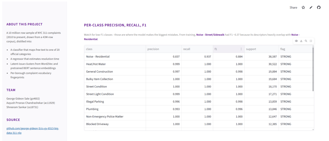
Figure 15: Bias Audit tab, lower half. Per-class precision, recall, F1, support, and a STRONG/WEAK flag for each of the top 20 complaint-type tags. The lone WEAK row in this run is Noise - Street/Sidewalk, which gets confused with Noise - Residential because the descriptor texts overlap. This is the documented reporting-bias finding the section anchors to (Kontokosta and Hong 2021).
