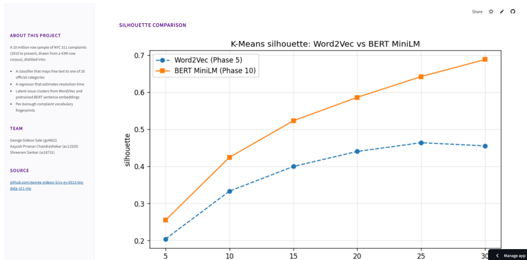
Figure 13: Cluster Atlas tab, silhouette comparison plot. K-Means silhouette across k from 5 to 30 for both embeddings: Word2Vec (Phase 5, dashed) and BERT MiniLM (Phase 10, solid). BERT outperforms Word2Vec at every k; the gap widens with larger k.
