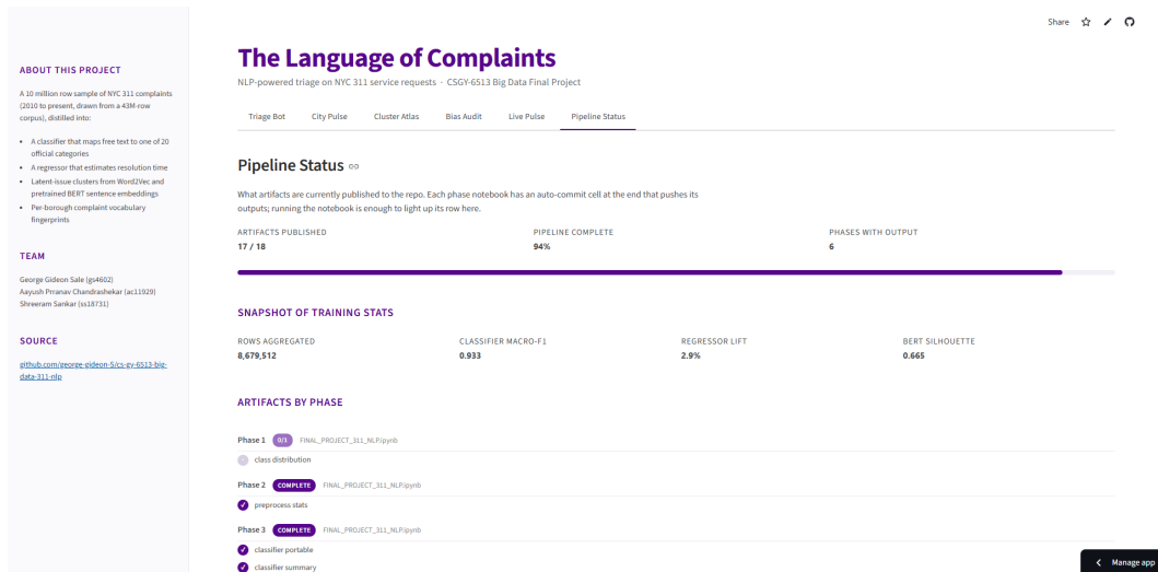
Figure 17: Pipeline Status tab, upper half. KPIs at the top: 17 of 18 artifacts published (94 percent), six of seven phases producing output. Snapshot training stats below: 8.68M rows aggregated, classifier macro-F1 0.933, regressor lift 2.9 percent, BERT silhouette 0.665. The artifacts-by-phase block begins below.
