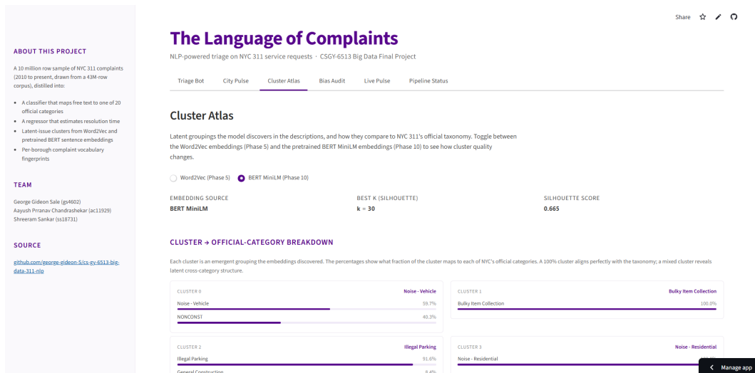
Figure 12: Cluster Atlas tab, BERT MiniLM mode. Same UI as the Word2Vec mode; embedding source toggles between the trained-from-scratch Word2Vec and the pretrained MiniLM encoder. Best k = 30 with silhouette 0.665 in this run, beating Word2Vec at the same k by approximately +0.20 absolute.
