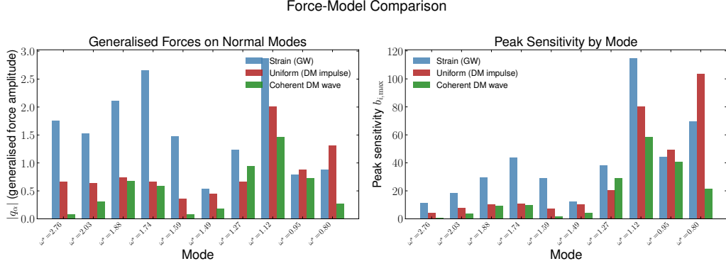
Figure 6: Per-mode generalized-force magnitudes |q_\alpha| (left) and peak sensitivities b_{\alpha,\max} (right) for all three driving models. The coherent DM wave produces the most balanced excitation across modes, which is reflected in its higher worst-case sensitivity in Table 3.
