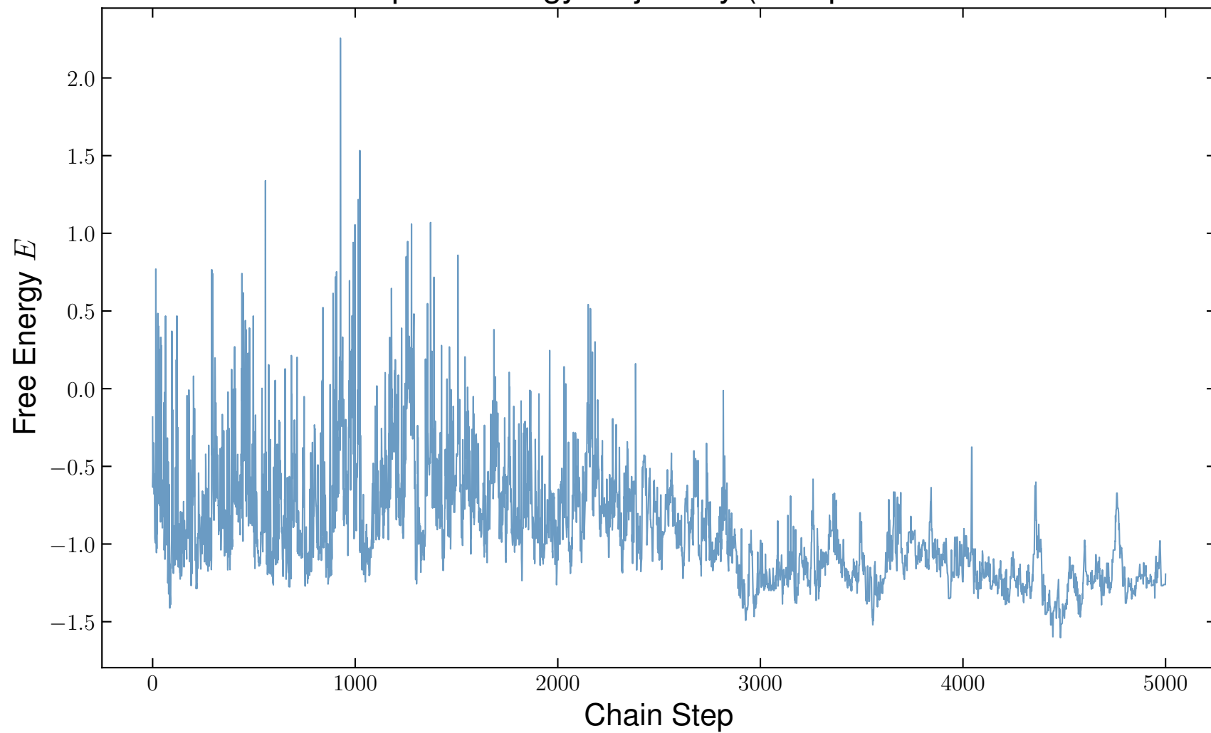
Metropolis Energy Trajectory (accept rate: 71.7)
