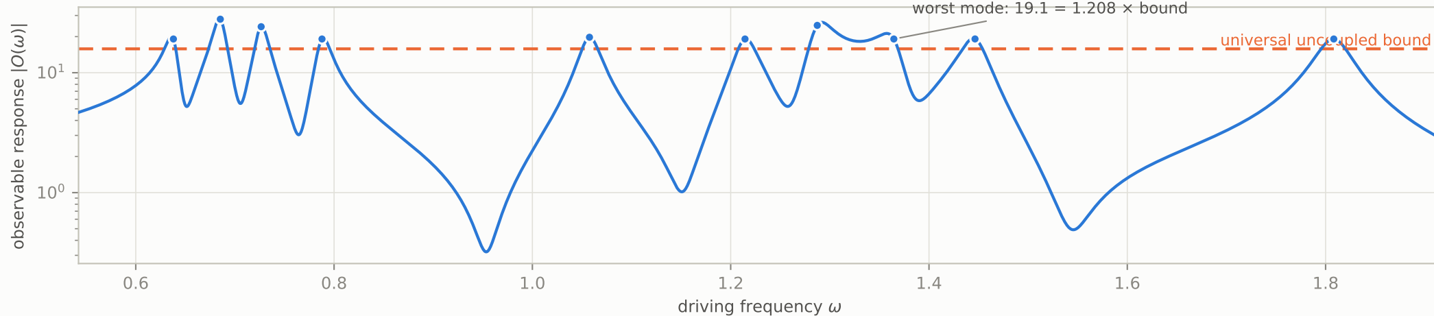
Swept response of the optimal observable — every resonance clears the bound
