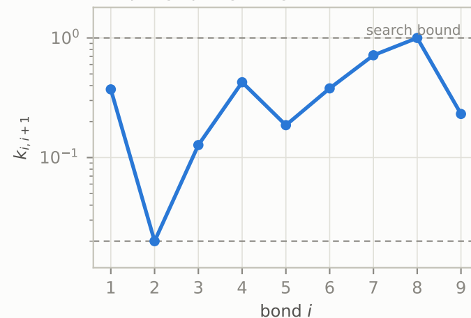
Coupling springs (log)
