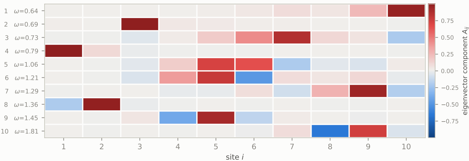
Normal-mode states
