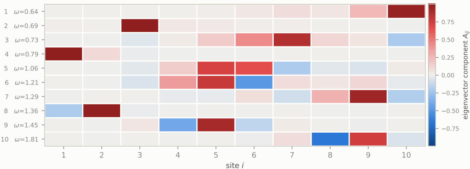
Normal mode states
