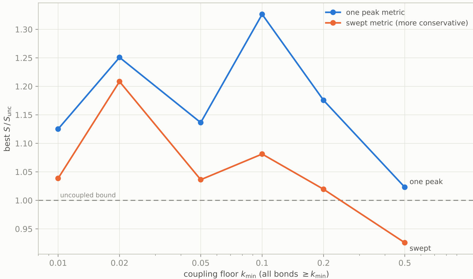
Best achievable sensitivity vs coupling floor
