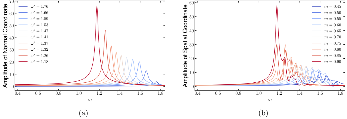
Figure 3: Forced-response amplitudes for the baseline system under GW strain driving. (a) Normal-coordinate amplitudes |b_i(\omega)| vs. driving frequency; each peak corresponds to one normal mode and its height gives b_{i,\max} . (b) Spatial (oscillator-level) amplitudes vs. frequency, showing which oscillators move most at each resonance.
