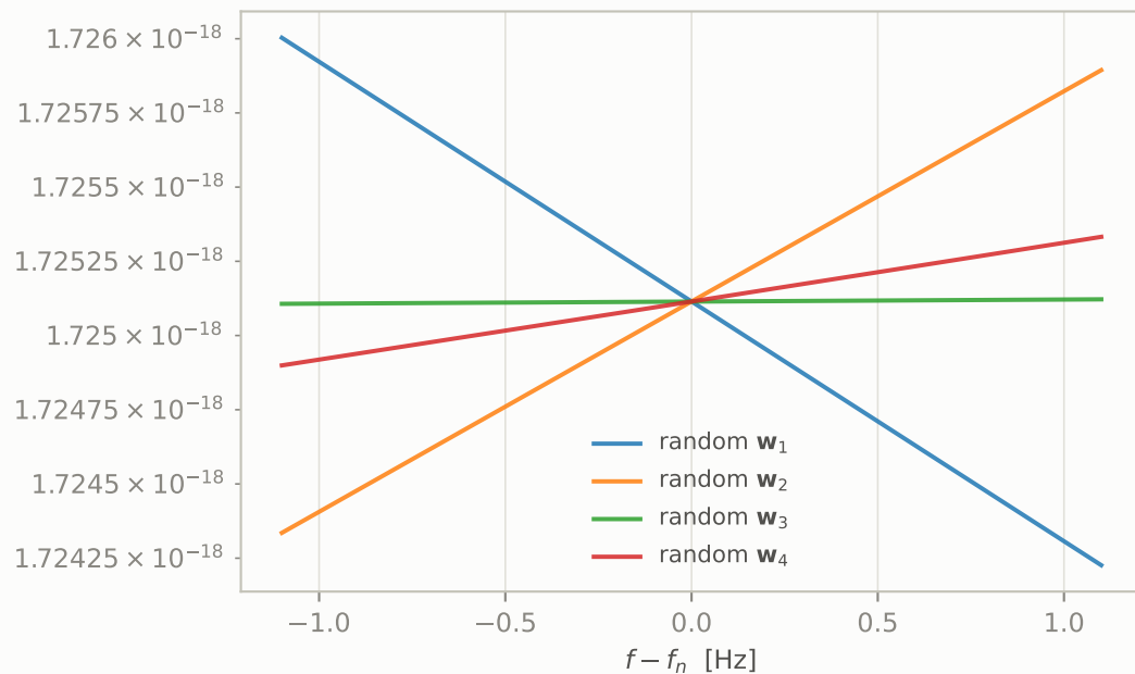
2) thermal \sqrt{S_h} on resonance is weight-independent (spread 7e-09)
