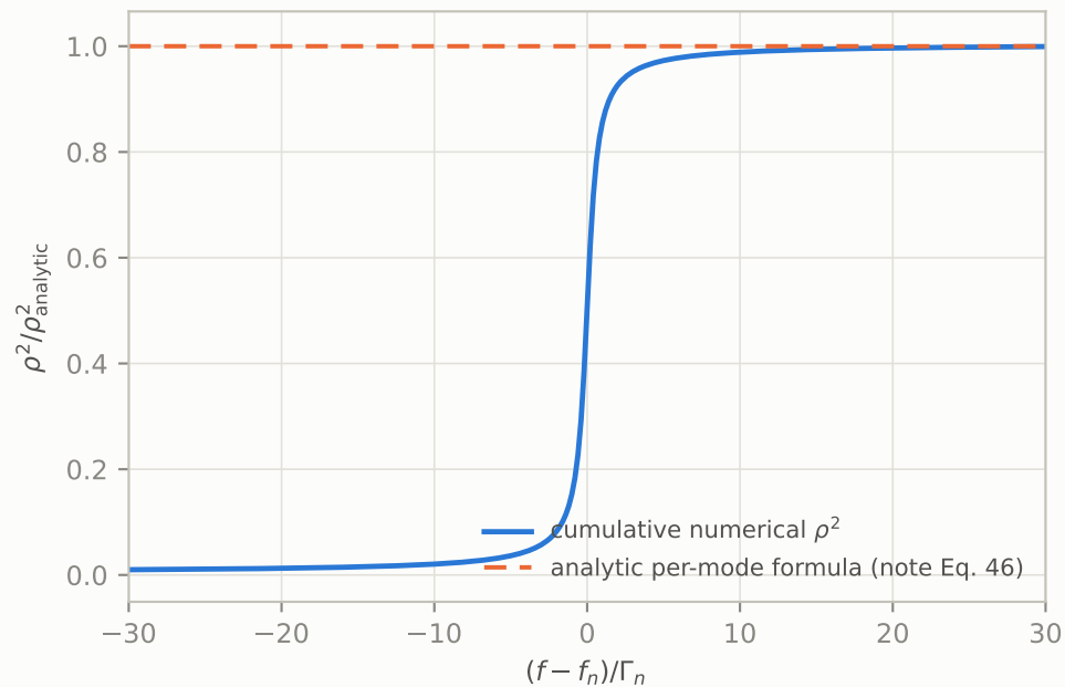
3) matched-filter SNR: numerical/analytic = 1.0075
