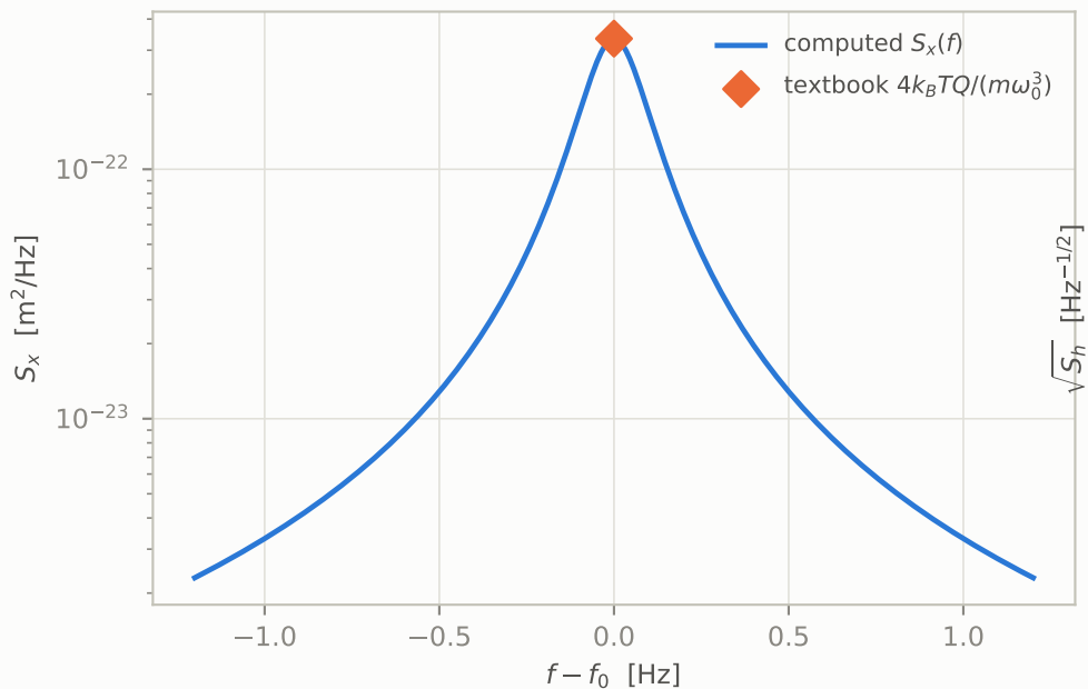
1) FDT thermal peak — agreement to 10^{-6}
