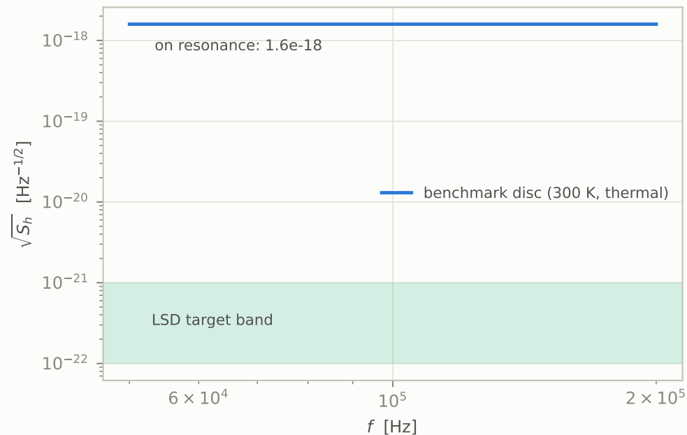
4) benchmark \sqrt{S_h} — gap = unconfirmed parameters
