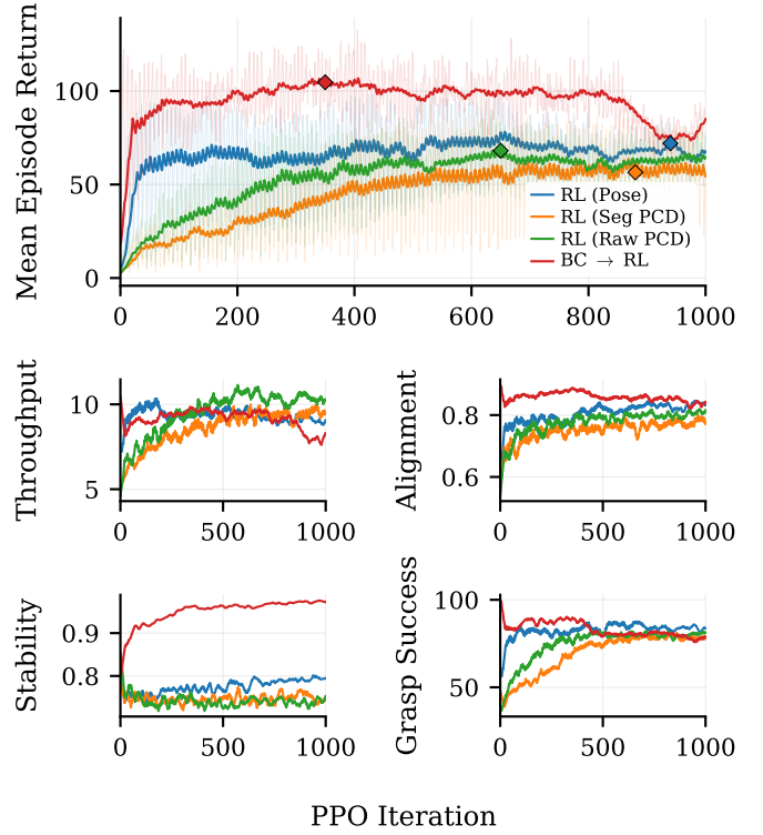
Fig. 2: PPO training curves. Mean episode return (the cumulative per-grasp reward r = g \cdot \alpha \cdot \varsigma summed over one 200-log clearing episode, averaged across N_{\text{env}} = 20 parallel environments) vs. PPO iteration. Each iteration collects 4N_{\text{env}} grasp cycles and performs one PPO update; bold lines show a 20-iteration rolling average with raw data in light shading. Diamond markers indicate the checkpoint selected for evaluation (highest mean return before degradation). Flat segments occur when no episode has terminated since the last update. All three from-scratch RL variants (Pose, Seg. PCD, Raw PCD) improve per-grasp reward but fail to achieve full pile clearing (Table IV). BC→RL initializes from the trained BC policy and reaches the highest mean return while maintaining near-complete clearing; performance degrades after \sim 500 iterations, motivating early stopping. Bottom panels decompose the reward signal into its per-grasp components.
