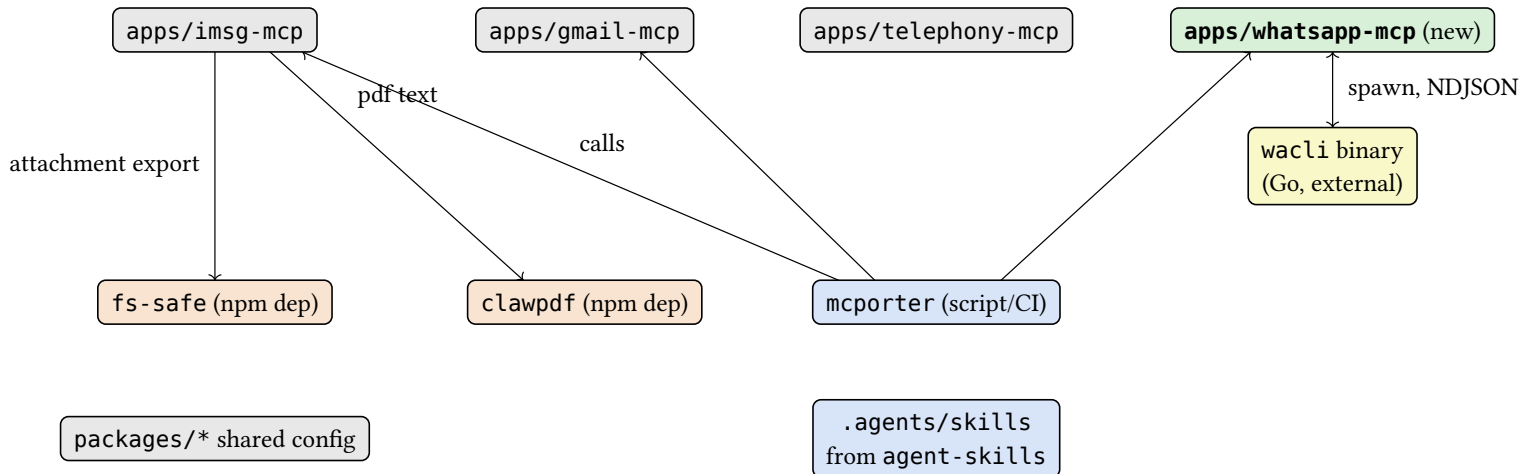
Figure 2: Proposed wiring. Only whatsapp-mcp is new code; the rest are dependencies or scripts.
