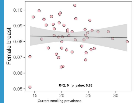
Correlation analysis
