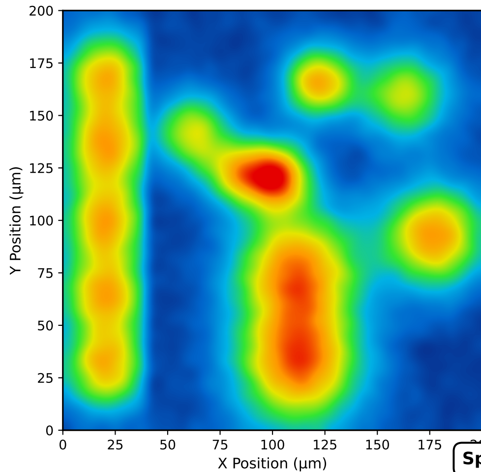
Spatial Accuracy of Long-Term Degradation Prognosis: (a) MF-DMF Prediction vs. Experimental Validation (SEM Experimental Data)
