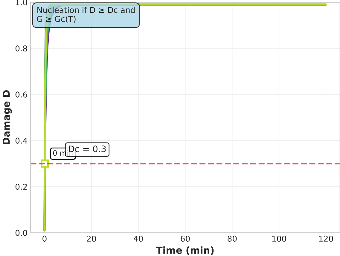
Panel B: Damage Evolution
