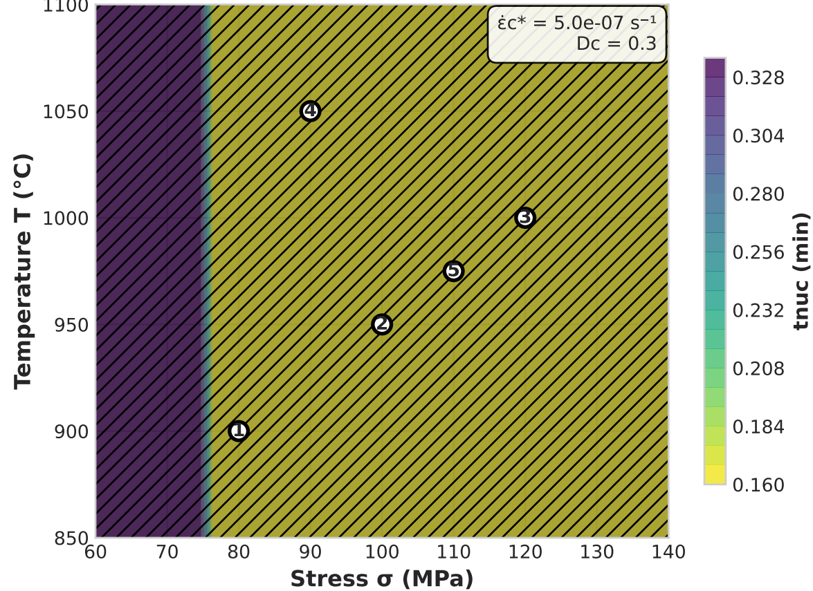
Panel C: \sigma -T Hazard Map
