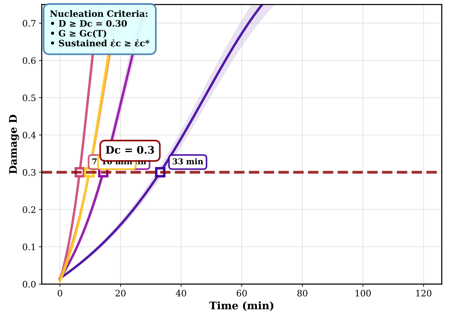
Figure 4a2: Creep Thresholds and Microcrack Initiation—Multi-Panel Synthesis
