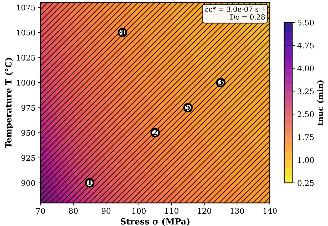
Panel C: \sigma -T Hazard Map
