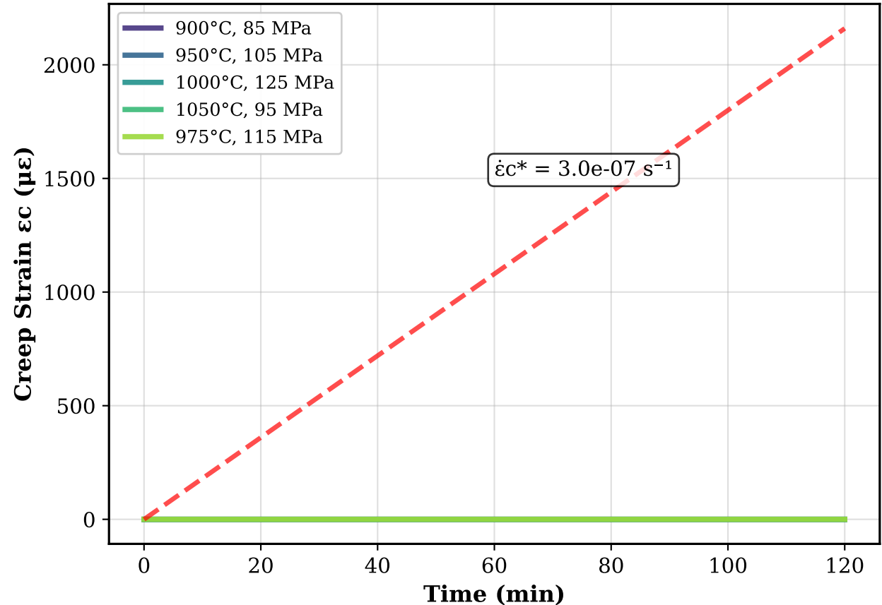
Panel A: Creep Strain Evolution
