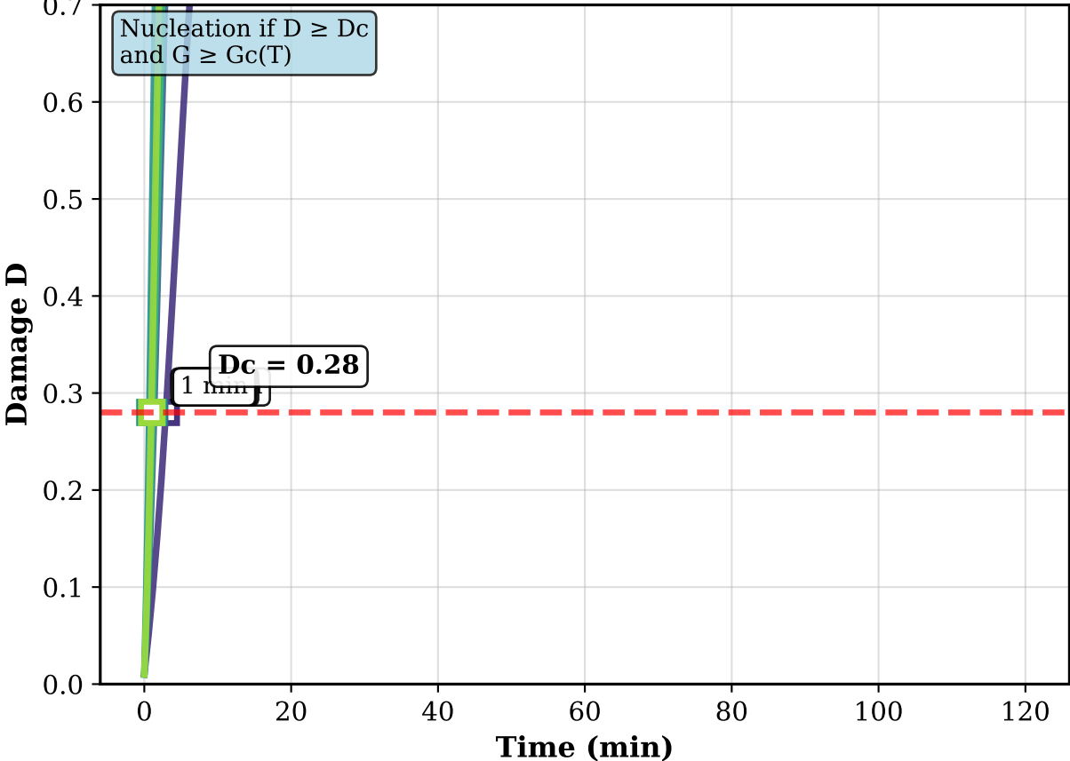
Panel B: Damage Evolution
