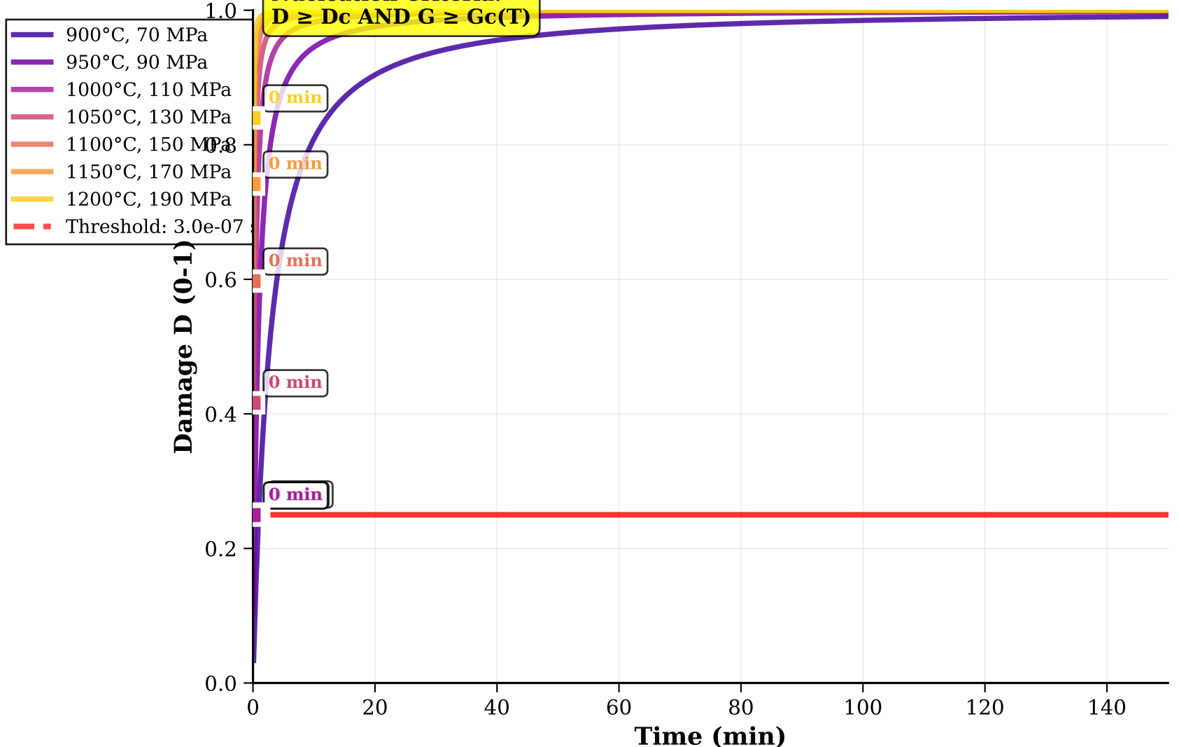
Figure 4a.2: Creep Thresholds and Microcrack Initiation Enhanced Multi-Panel Synthesis with Model Validation
