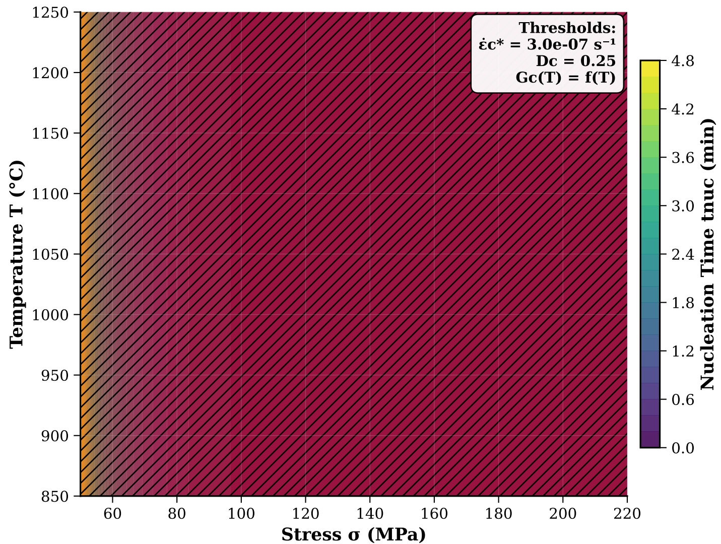
Panel C: \sigma -T Hazard Map (Operating Envelope)
