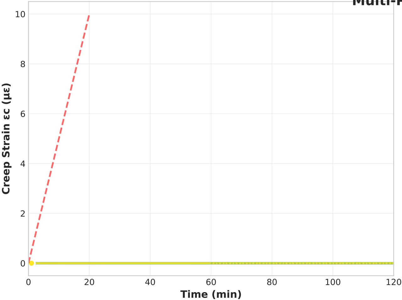
Figure 4a.2: Creep Thresholds and Microcrack Initiation
