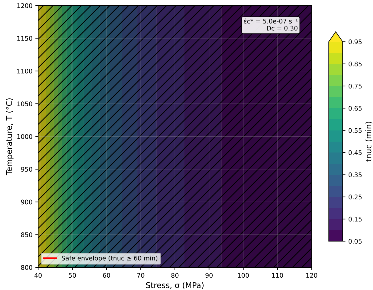
\sigma -T Hazard Map (Operating Envelope)
