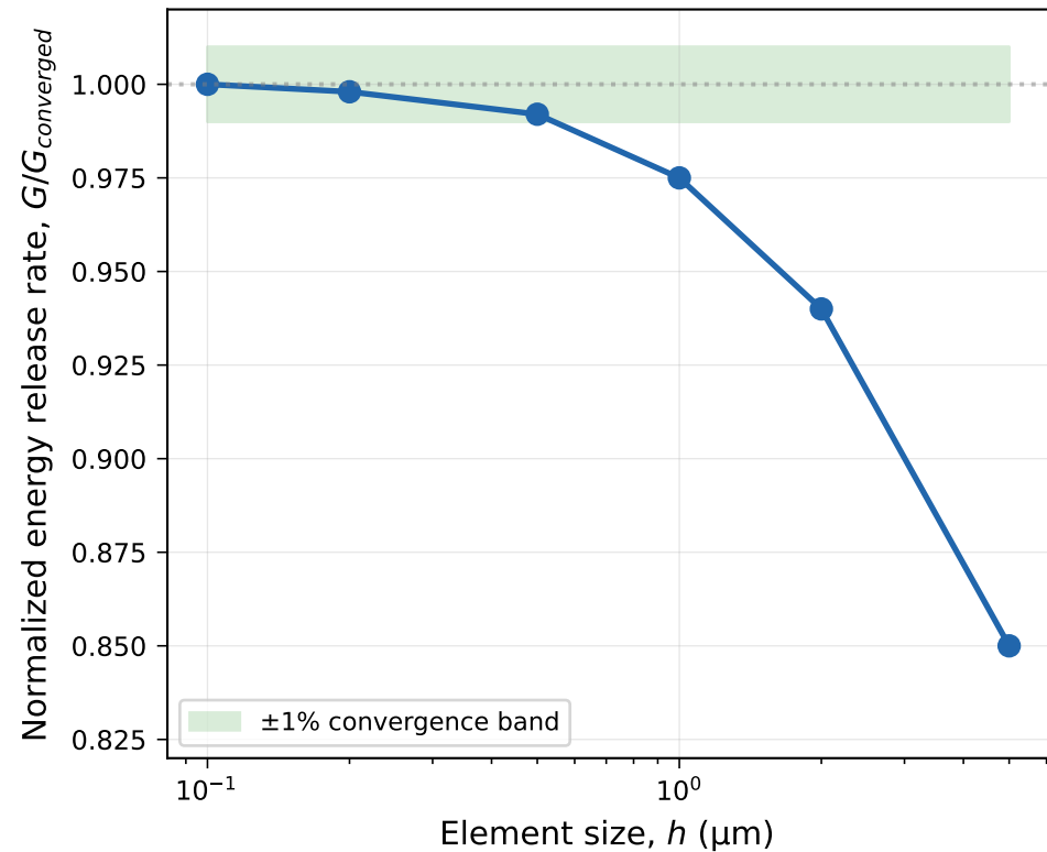
(a) Mesh Objectivity: Energy Release Rate
