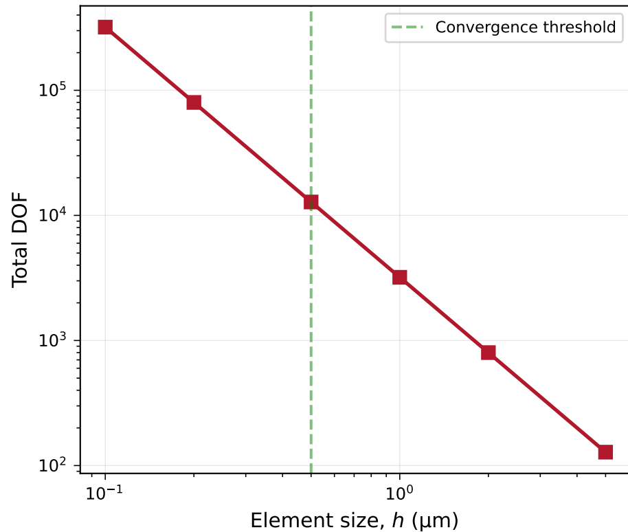
(b) Computational Cost: DOF vs Mesh Size
