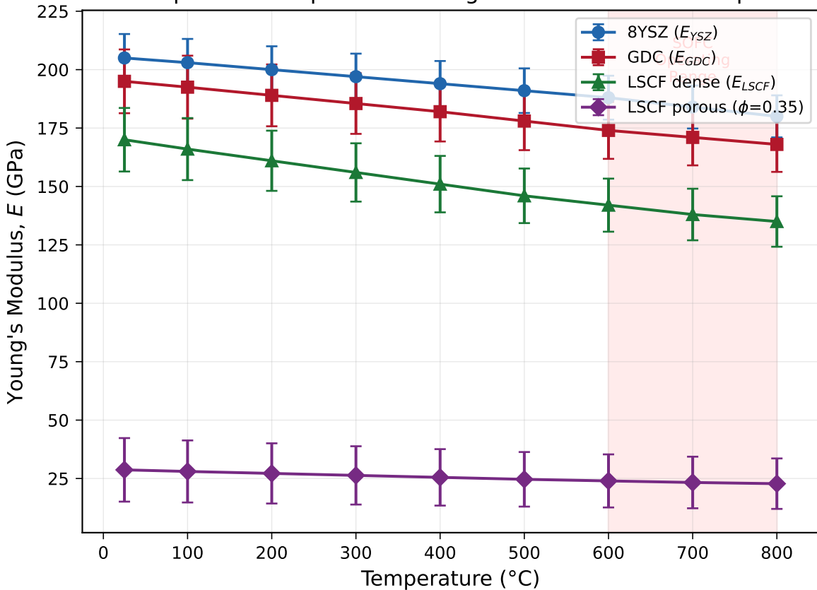
Temperature-Dependent Young's Modulus for UMAT Input
