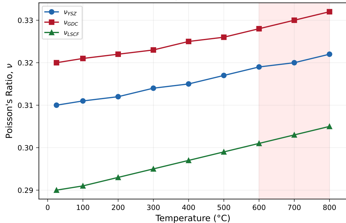
Temperature-Dependent Poisson's Ratio
