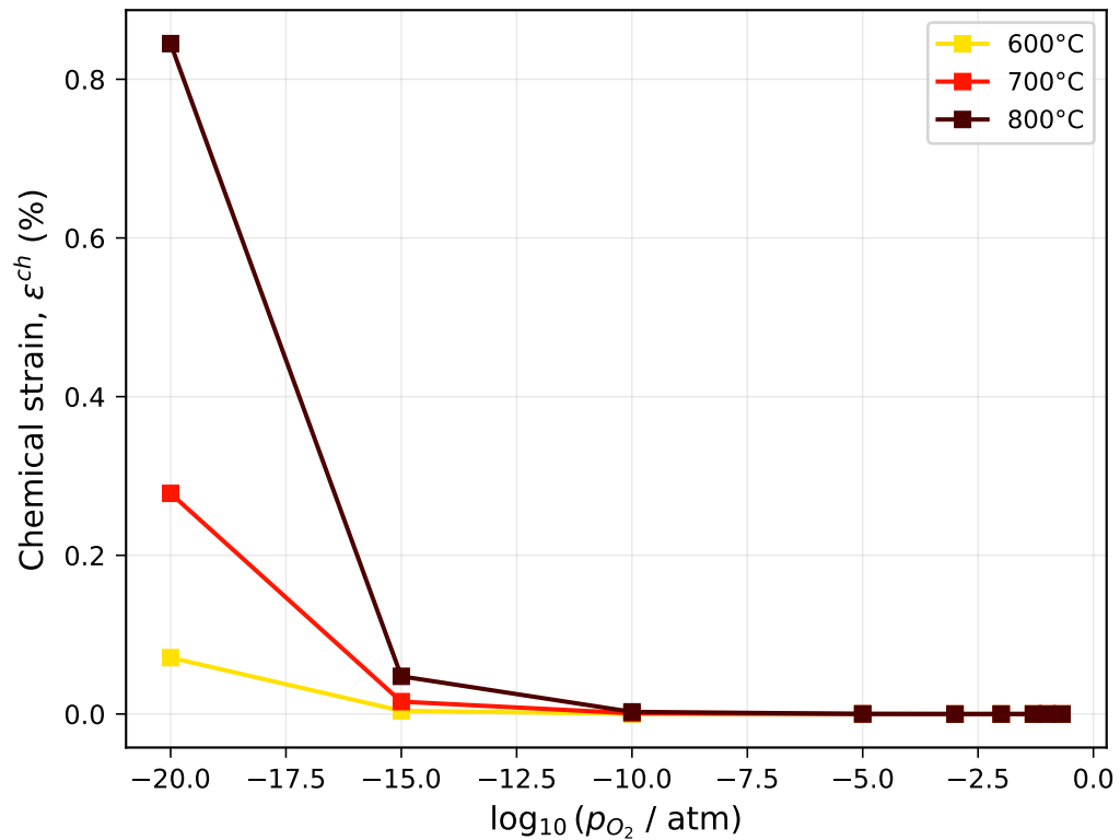
(b) GDC: \varepsilon_{iso}^{ch} vs p_{O_2}
