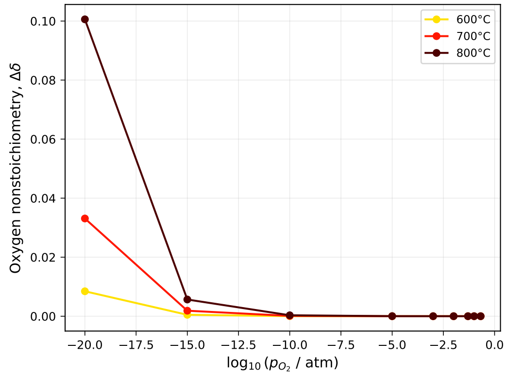
(a) GDC: \Delta\delta vs p_{O_2}
