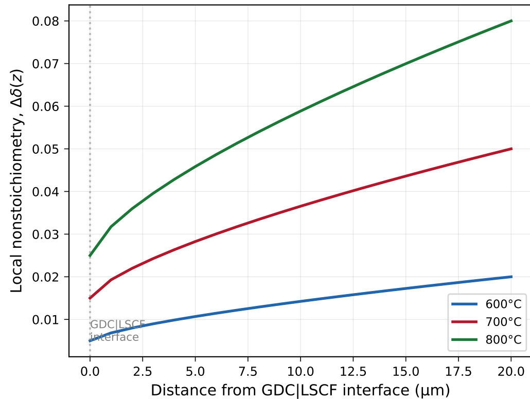
(a) \Delta\delta Profile across LSCF Cathode
