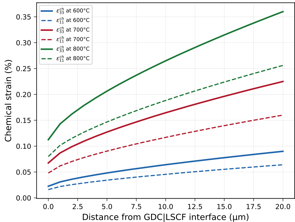
(b) Chemical Strain Profile across LSCF
