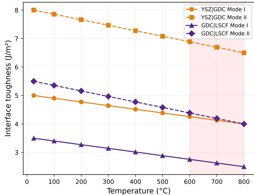
(a) Interface Toughness: G_{c,I} and G_{c,II} vs T
