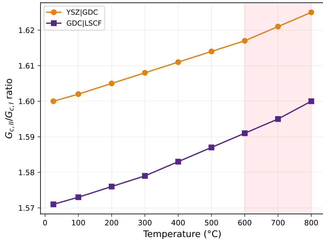
(b) Mode II/Mode I Toughness Ratio vs T
