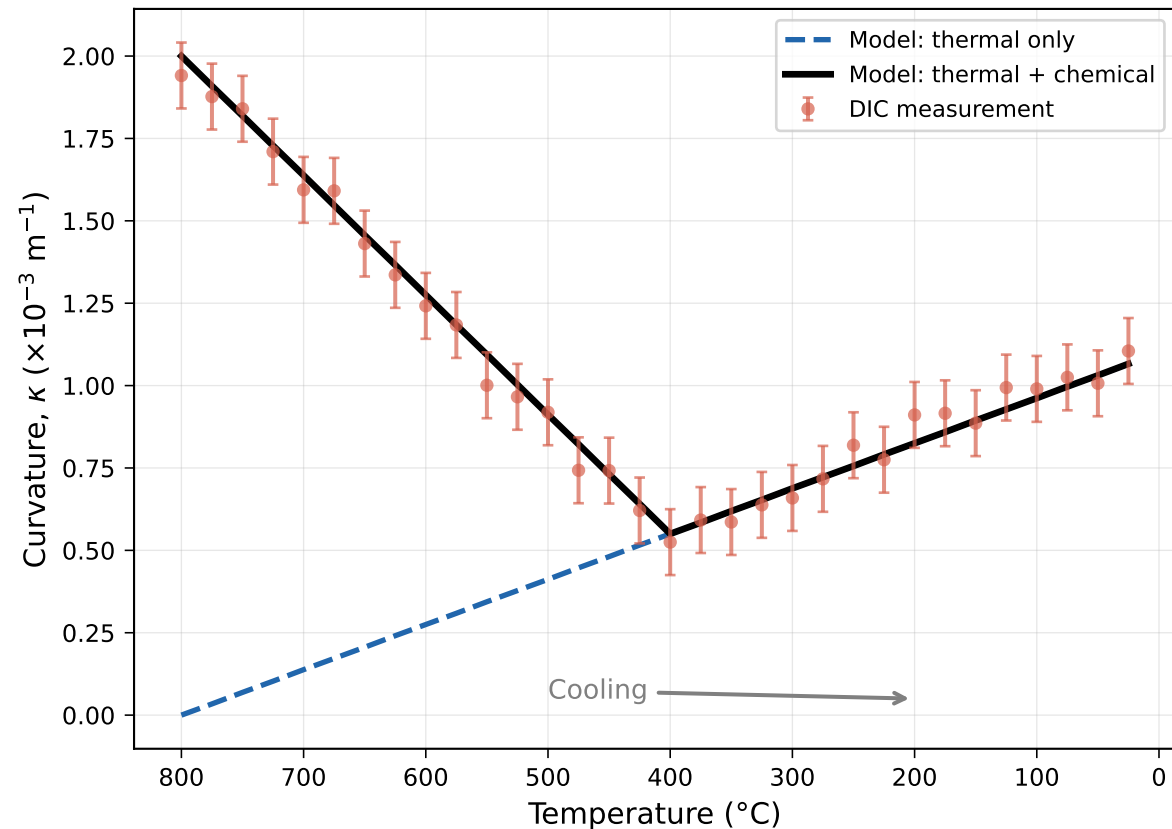
Global Curvature Evolution \kappa(T) During Cooling
