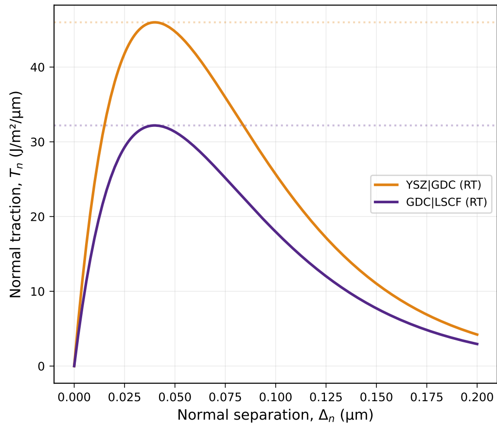
(a) Mode I: T_n(\Delta_n)
