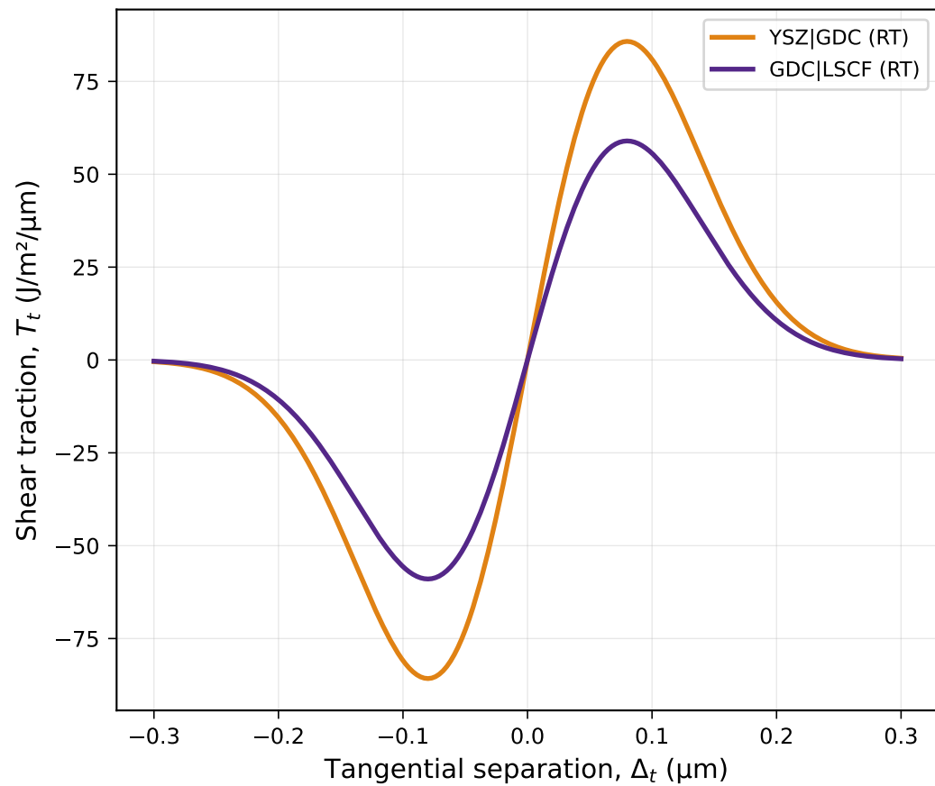
(b) Mode II: T_t(\Delta_t)
