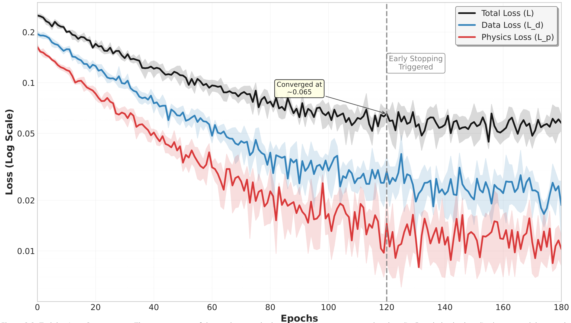
Figure 2.2: Training Loss Convergence. The convergence of the total composite loss ( L ) and its components—data loss ( L_d ) and physics loss ( L_p )—over training epochs. The model shows rapid initial improvement followed by stable convergence. The vertical dashed line at epoch 120 indicates the point of early stopping, preventing overfitting. The shaded regions represent \pm 1 standard deviation from 5 independent training runs, demonstrating the robustness of the training protocol and the reproducibility of the loss minimization.
