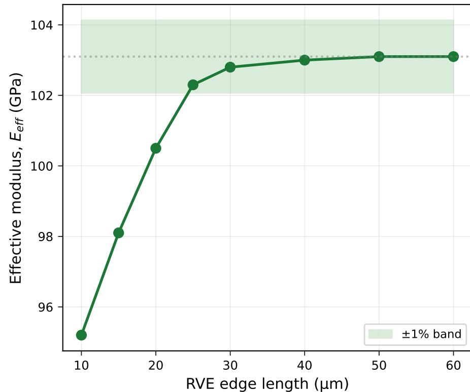
(a) RVE Convergence: E_{eff} (LSCF, \phi=0.35 )
