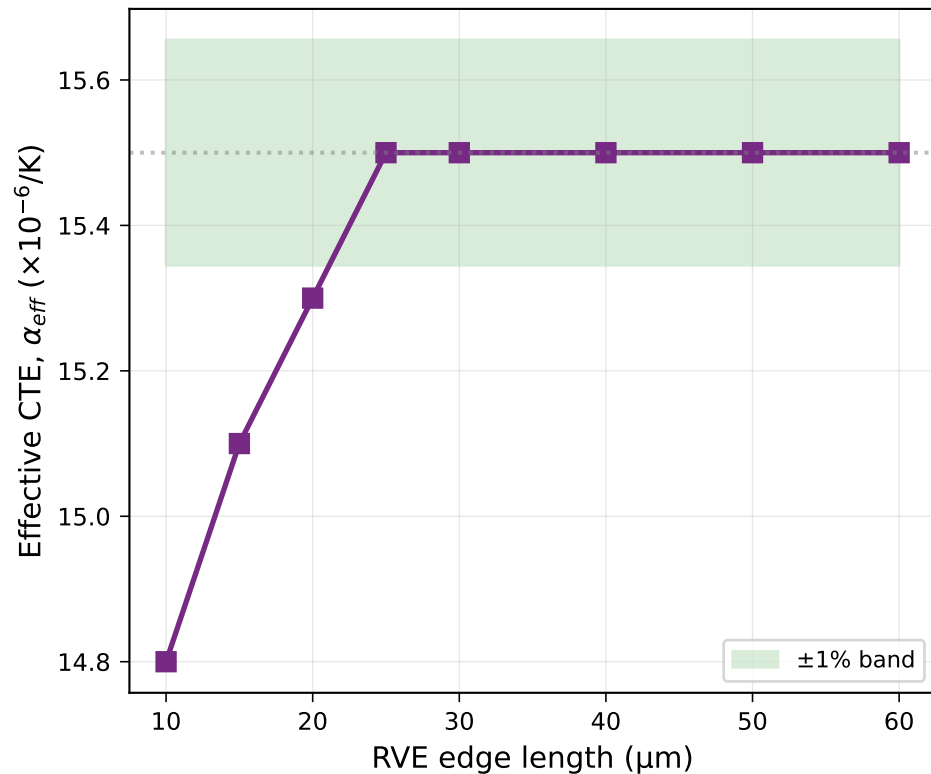
(b) RVE Convergence: \alpha_{eff} (LSCF, \phi=0.35 )
