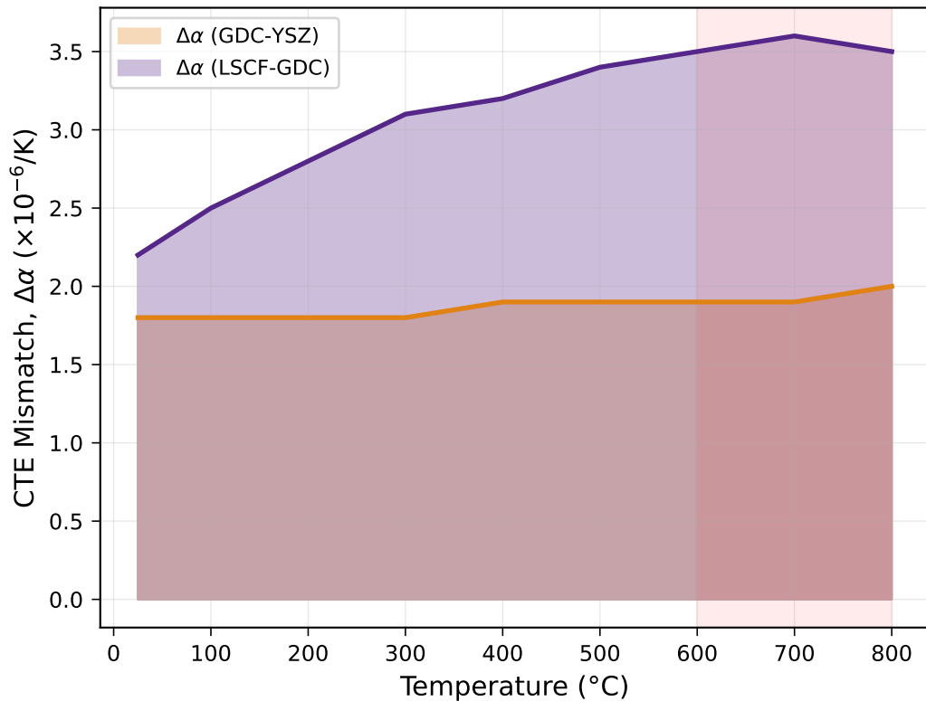
(b) Interface CTE Mismatch (Driving Force)
