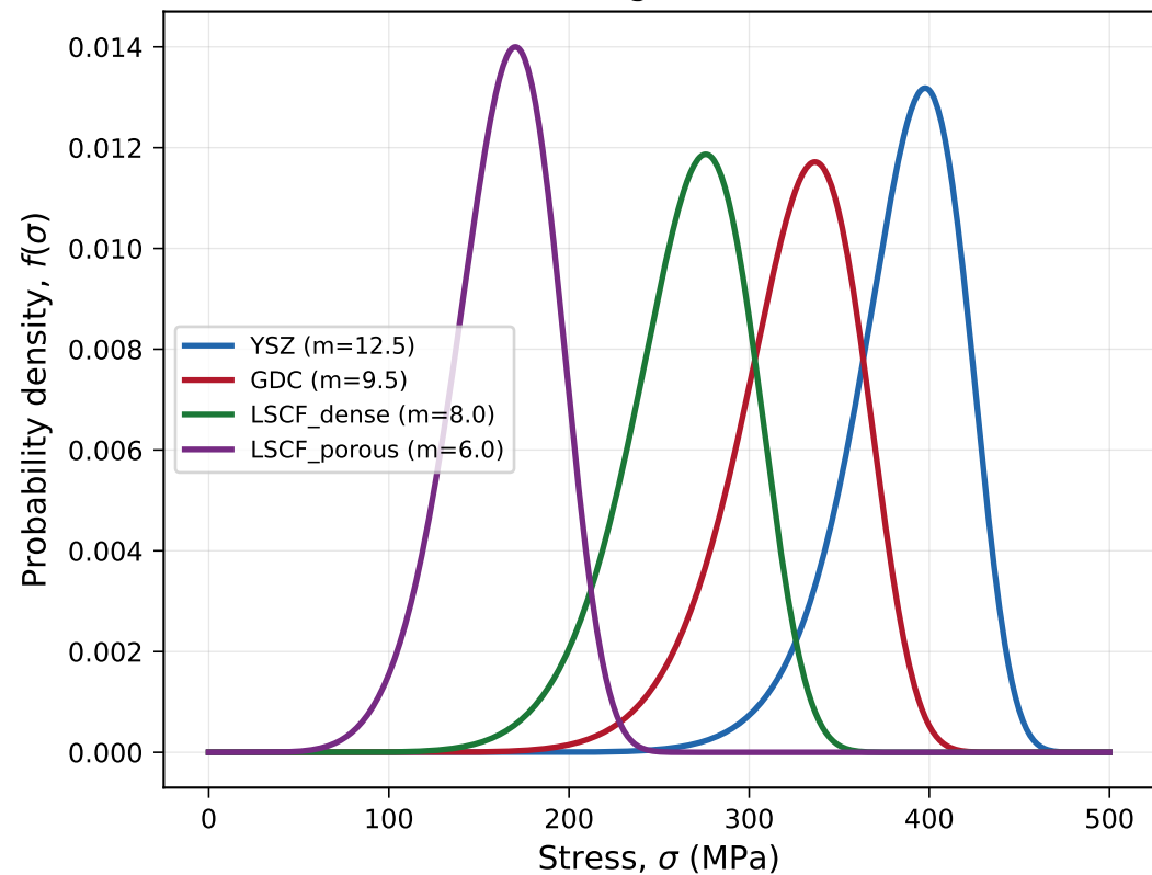
(a) Weibull Strength Distribution (RT)
