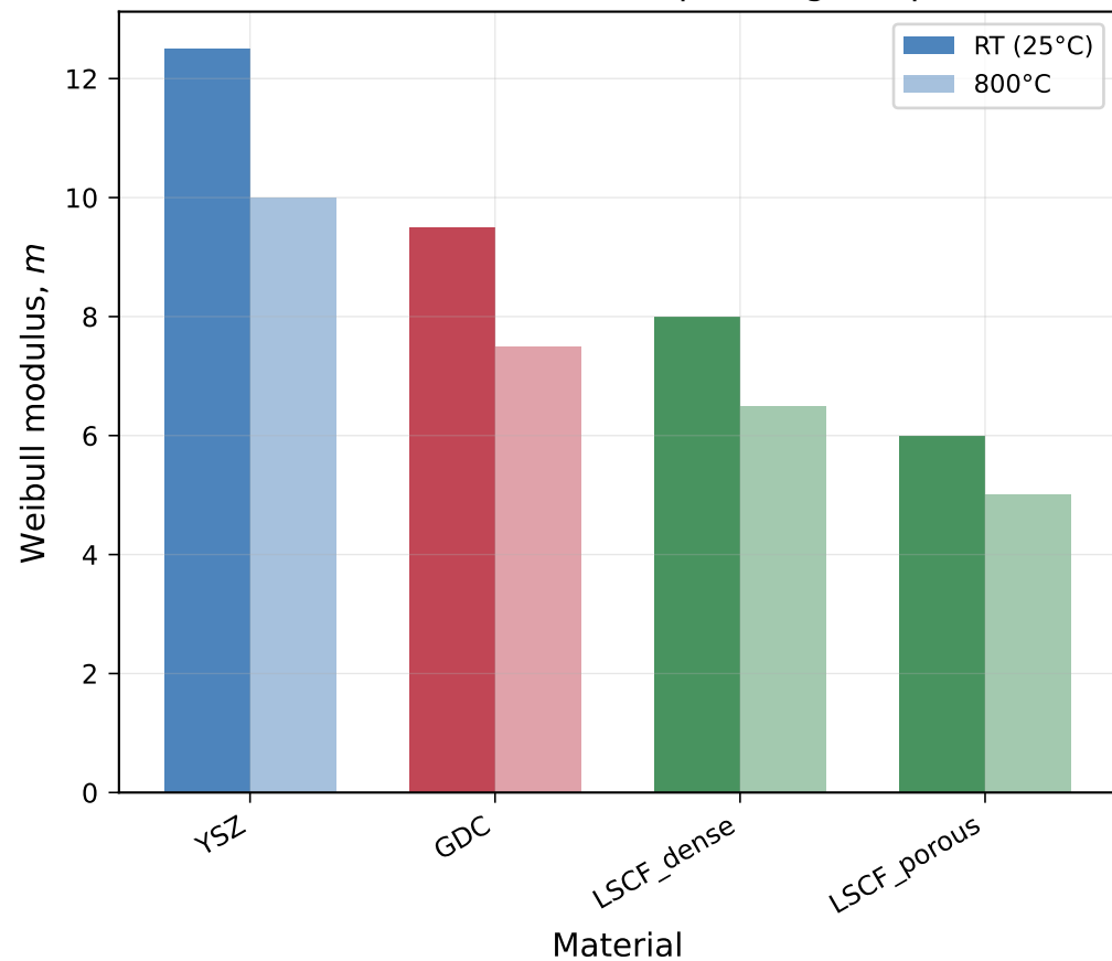
(b) Weibull Modulus: RT vs Operating Temperature
