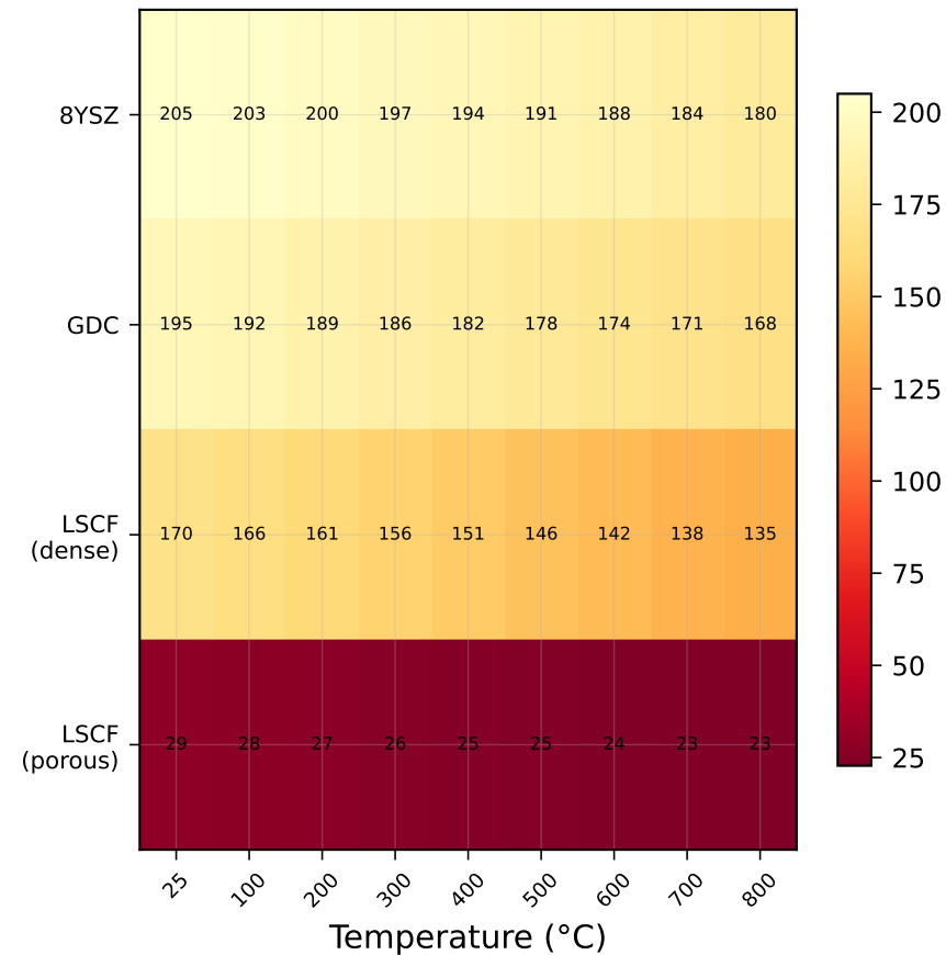
(a) Young's Modulus E (GPa)
