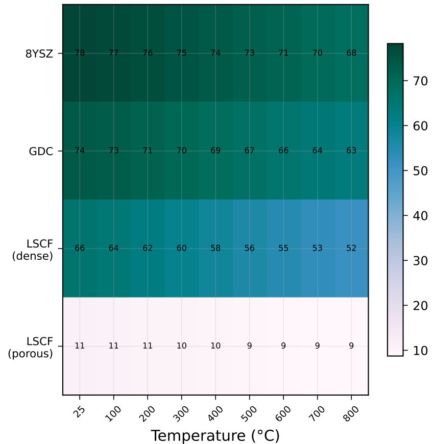
(c) Shear Modulus \mu (GPa)
