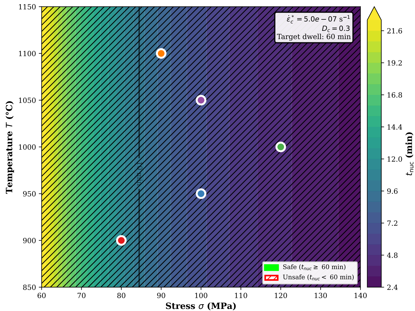
Panel C: \sigma - T Hazard Map and Operating Envelope
