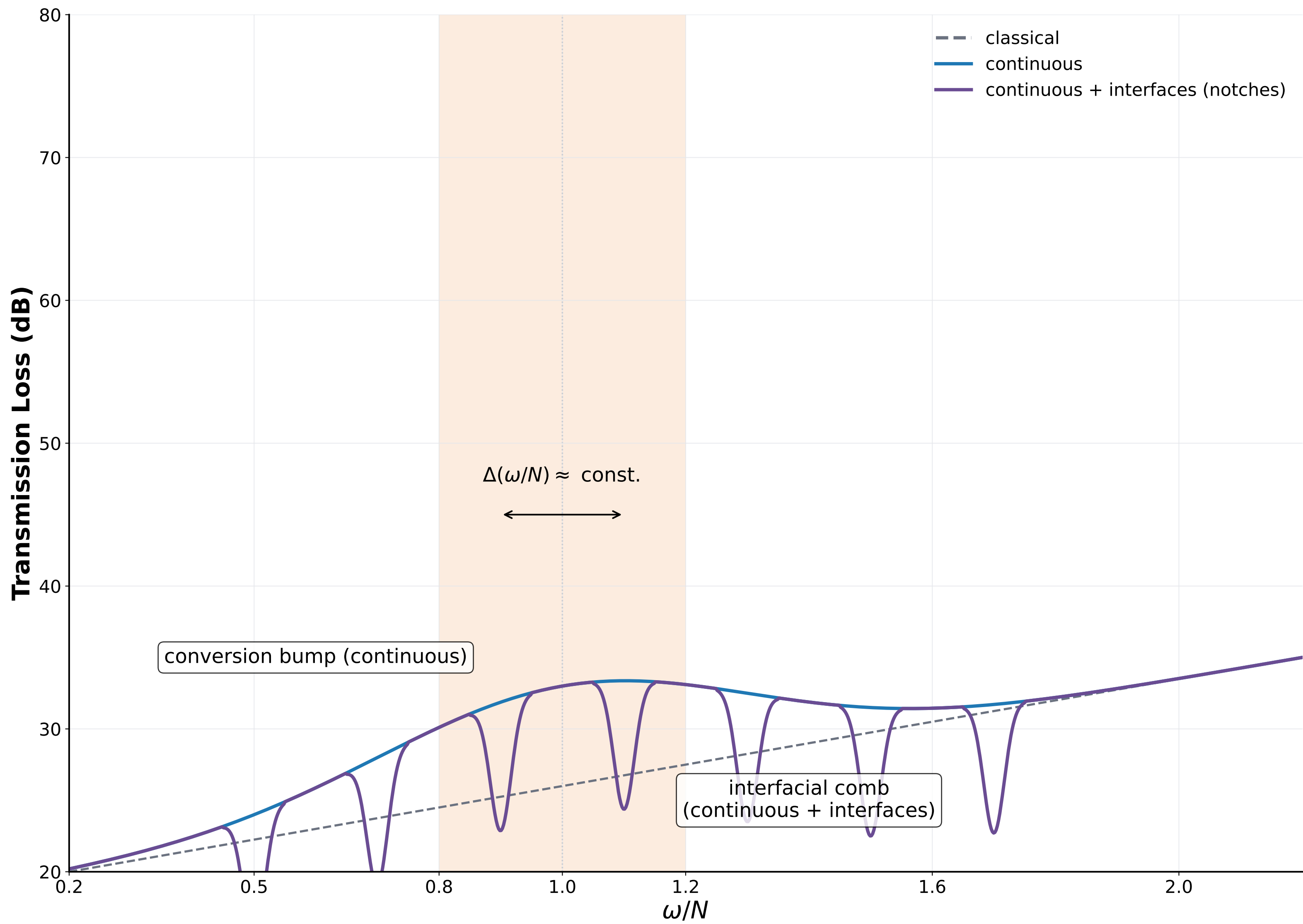
Figure 3.9A. Frequency-sweep signatures: a broad conversion bump at \omega/N \approx 1 for continuous stratification; adding sharp interfaces imposes narrow spectral notches on top of the bump.
