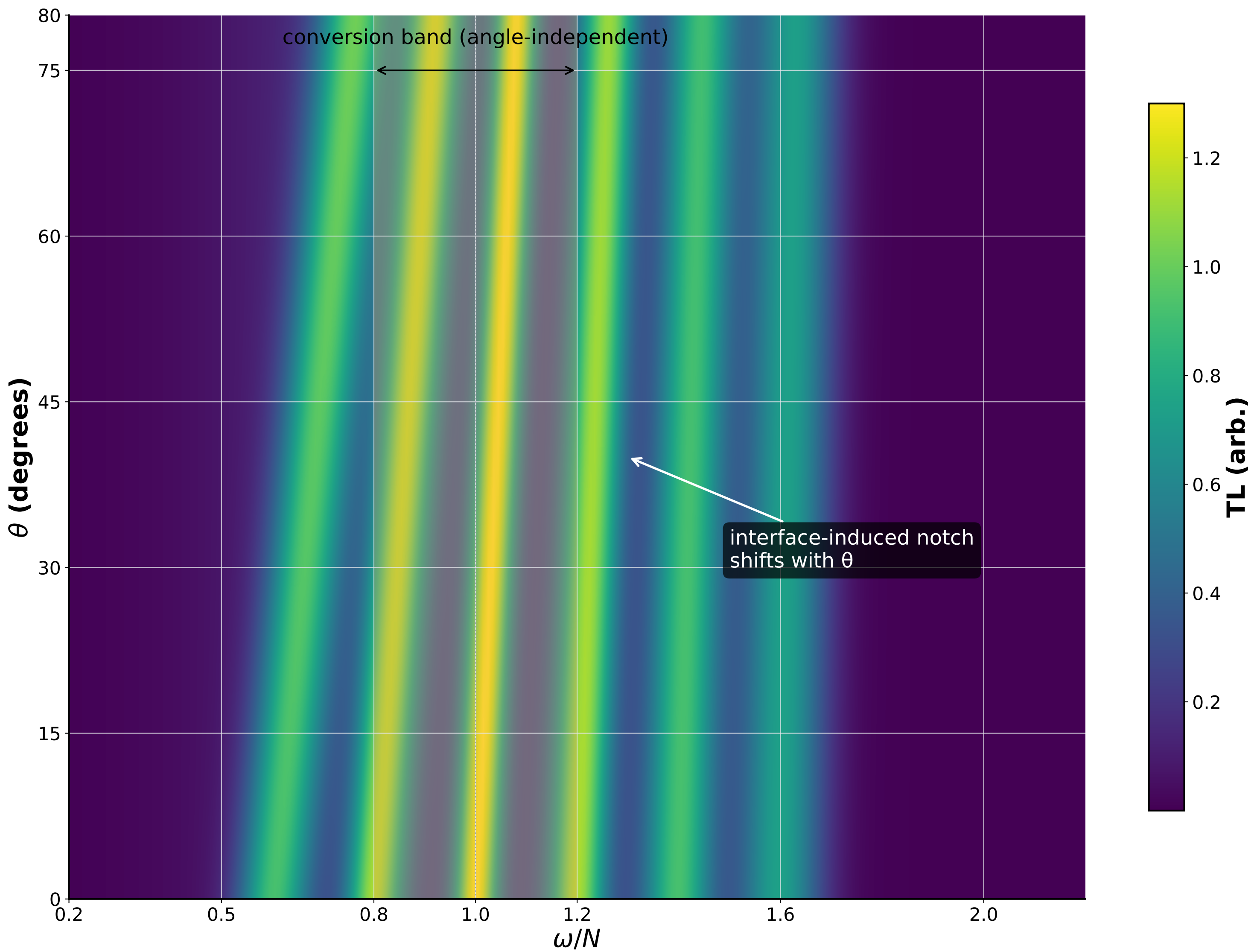
Figure 3.9B. Angle-frequency plate: interface-induced notches shift with angle, while the conversion band remains centered at \omega/N \approx 1 .
