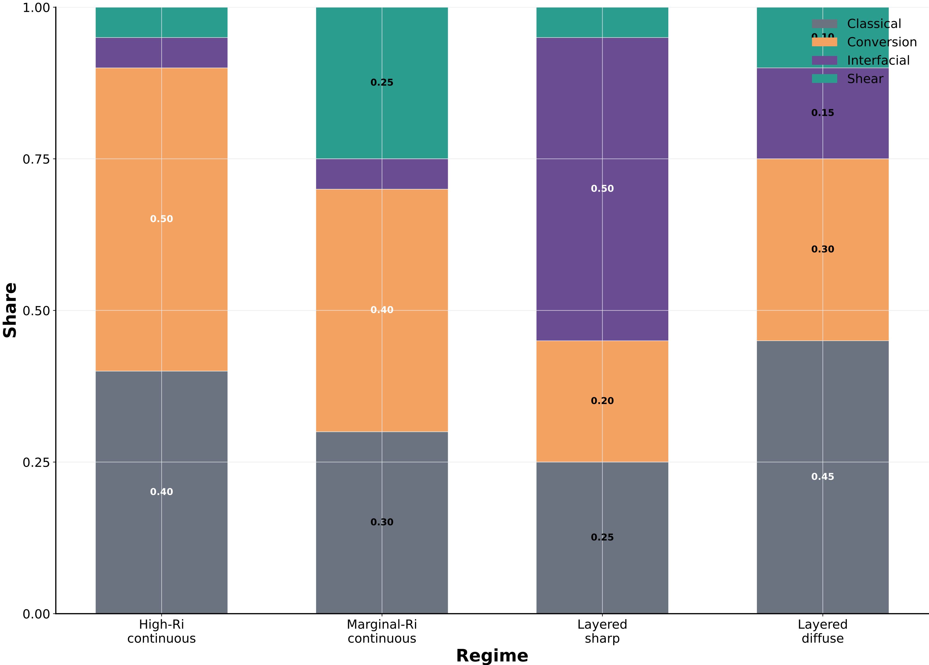
Figure 3.9D. Mechanism shares (summing to unity) for four regimes: conversion dominates high-Ri continuous; shear rises under marginal Ri; interfacial loss peaks for layered sharp and weakens for layered diffuse.
