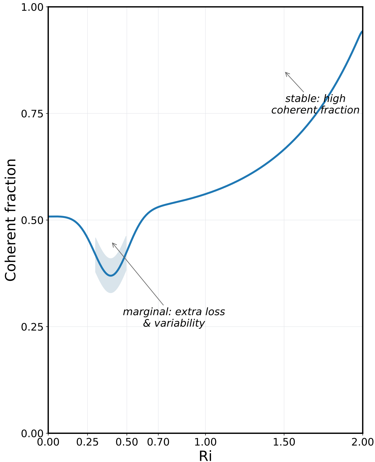
Figure 3.6C — Coherence loss and spectral broadening with decreasing Ri
