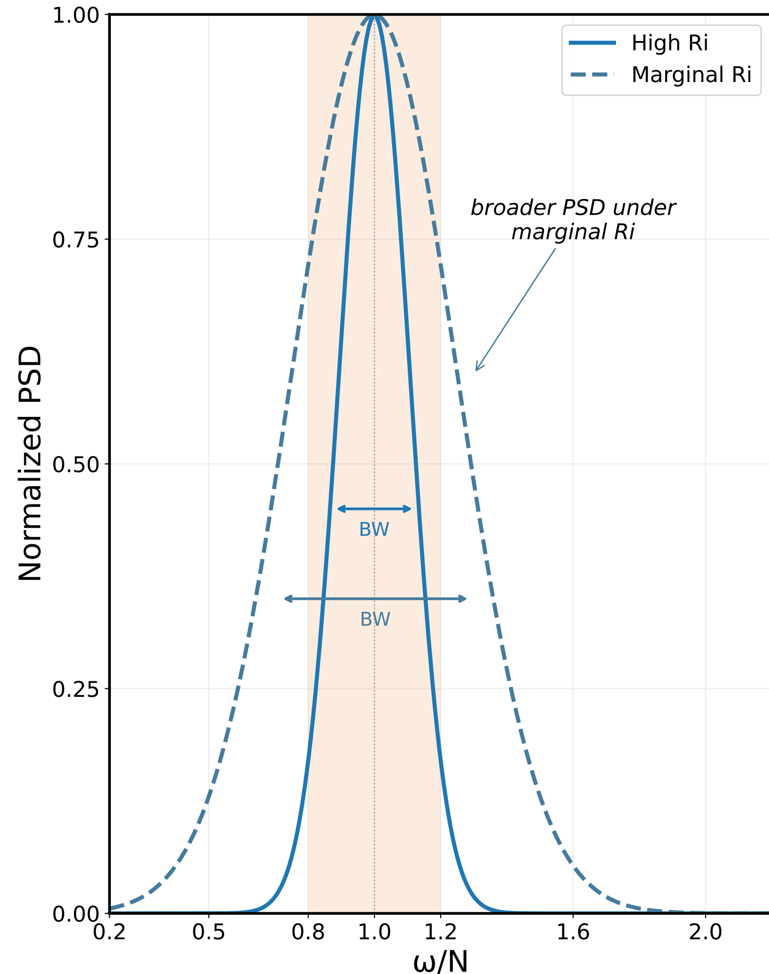
Figure 3.6C — Coherence loss and spectral broadening with decreasing Ri
