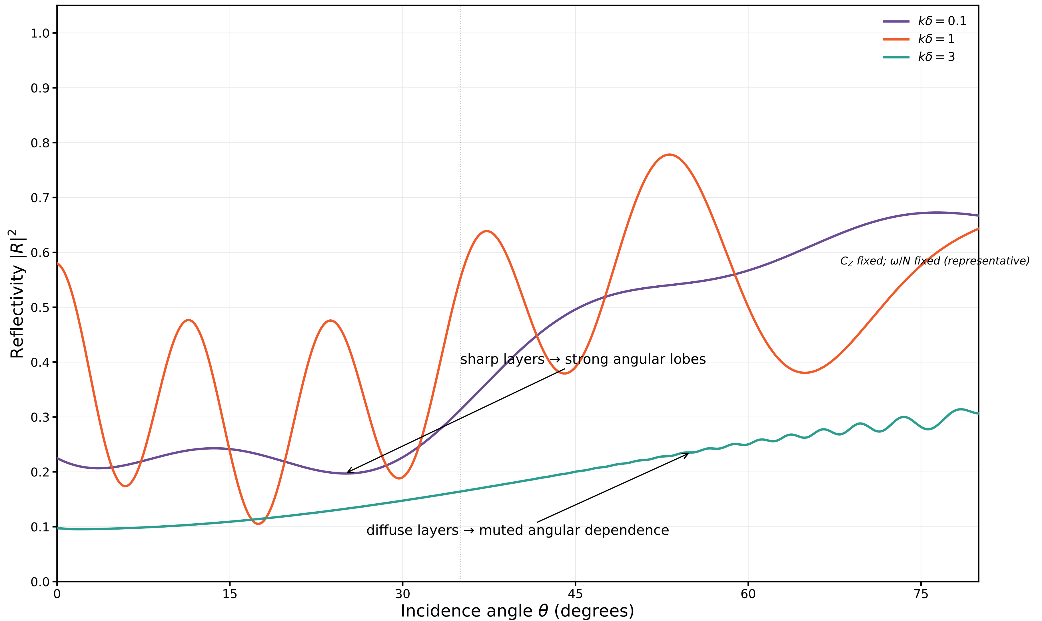
Figure 3.5C. Reflectivity vs incidence for thickness parameter k\delta at fixed contrast. Thin/sharp layers yield pronounced obliquity-dependent lobes; diffuse layers produce smoother, muted trends.
