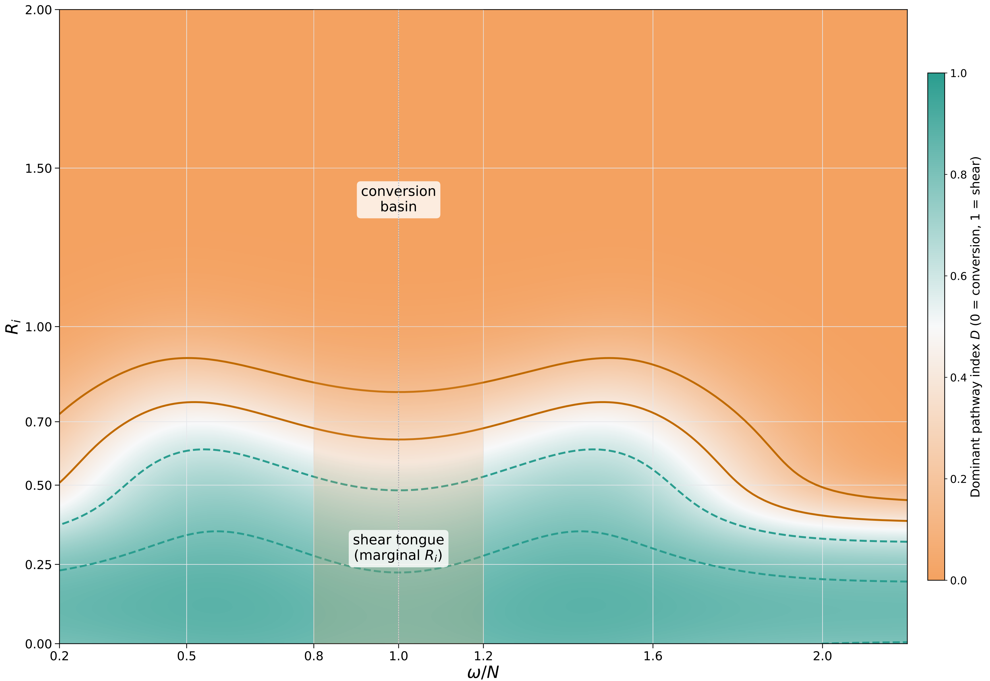
Figure 3.8A. Predicted dominant pathway map for continuous stratification. Conversion dominates near \omega/N \approx 1 at higher R_i ; shear dominates under marginal R_i , especially around the conversion band.
