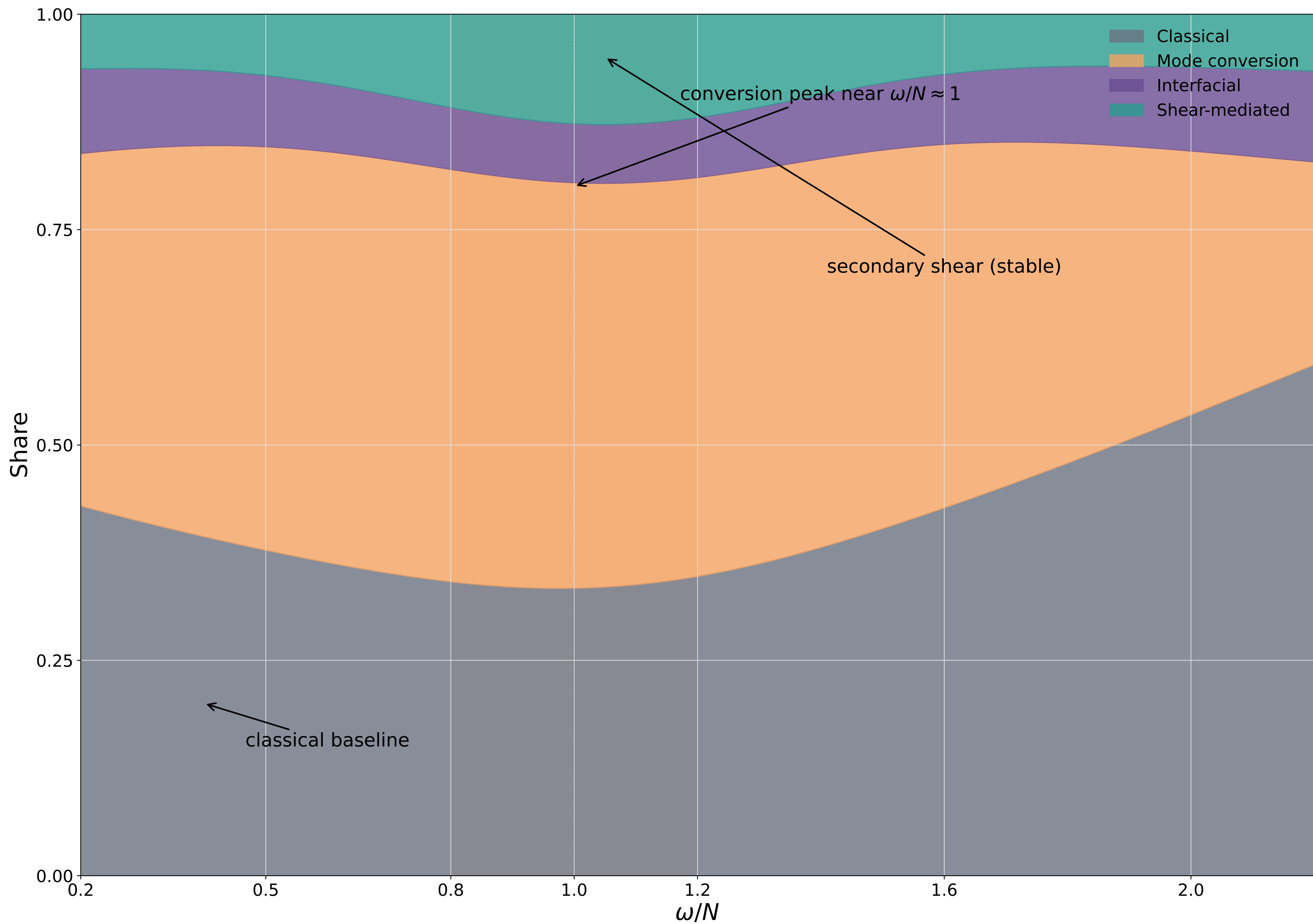
Figure 3.7B1 — Mechanism shares vs \omega/N (High R_i , continuous)
