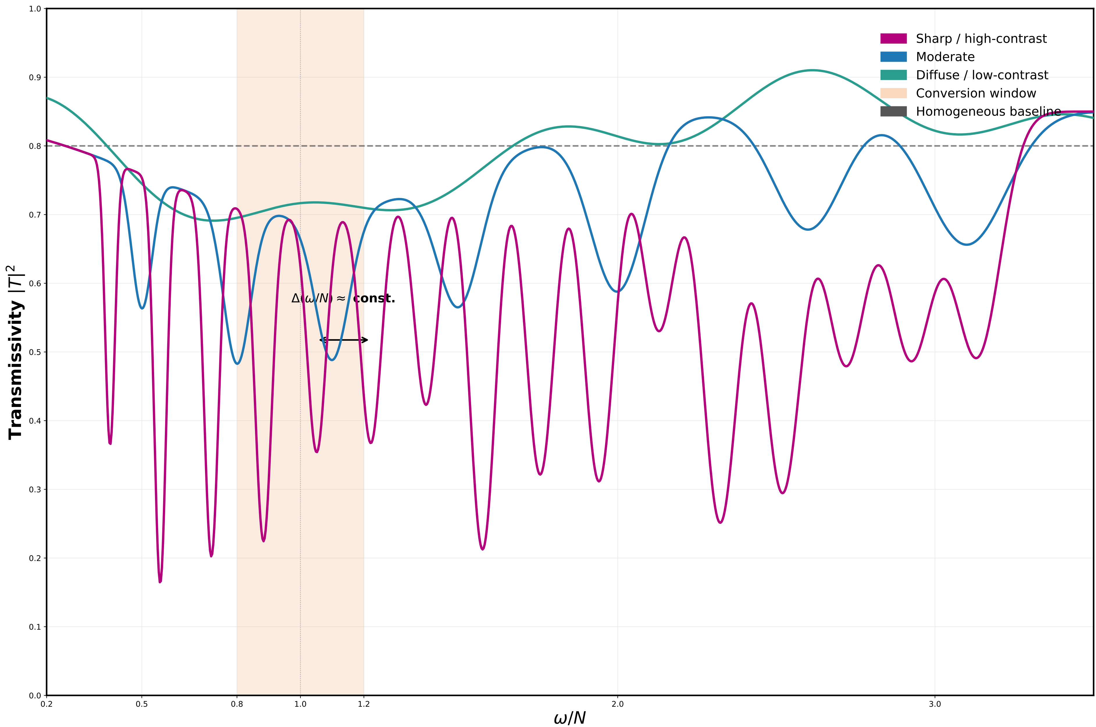
Figure 3.5B. Transmissivity vs normalized frequency across interface regimes. Sharp, high-contrast layers exhibit deep, frequent notches; moderate layers show gentler quasi-periodic structure; diffuse/low-contrast layers are nearly smooth.
